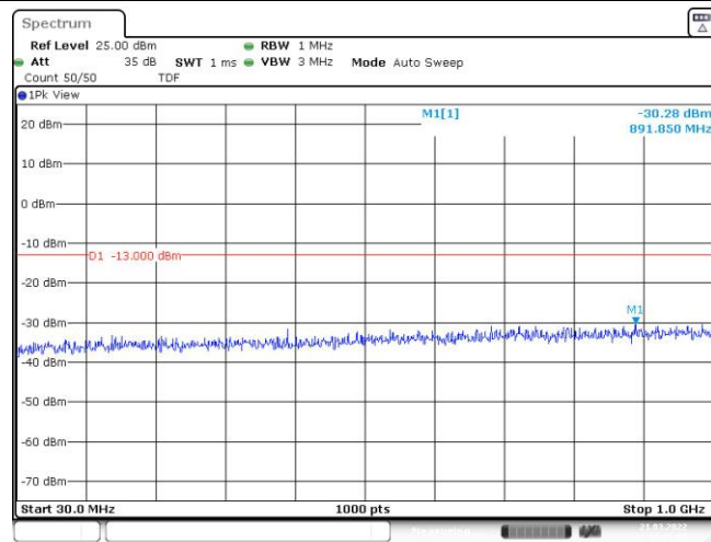
Band66-1.4MHz-QPSK-132322-1RB#0-Range1:30~1000MHz
