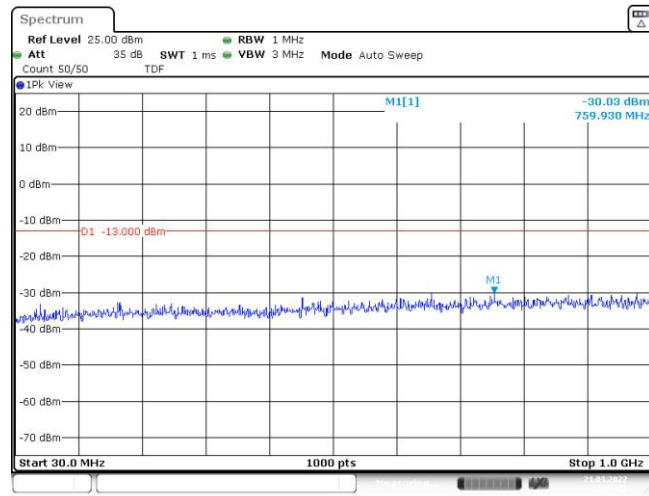
Band66-1.4MHz-QPSK-131979-1RB#0-Range1:30~1000MHz
