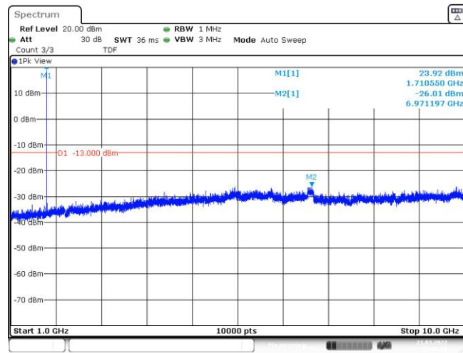
Band66-1.4MHz-QPSK-131979-1RB#0-Range2:1000~10000MHz
