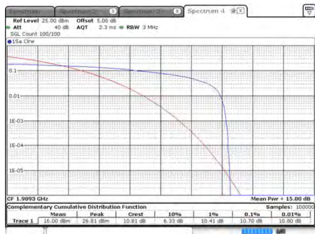
Cat M1_Band 2_CH19193_1.4M_QPSK_1RB0
