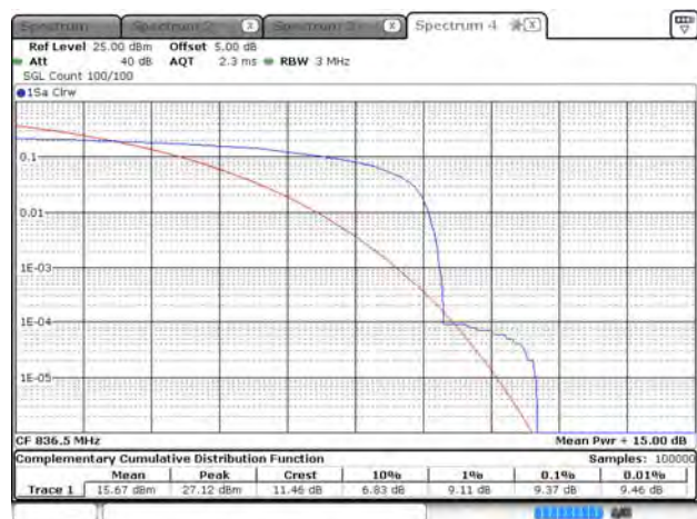
Cat M1_Band 26_CH26915_3M_QPSK_1RB0
