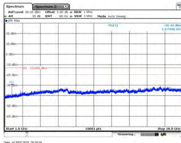
Band 5_CH20525_3M_1RB0_QPSK_Above 1G
