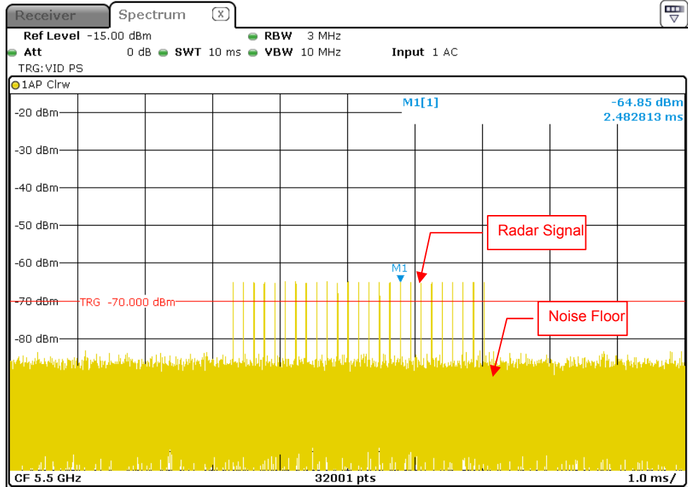
Radar Signal 2
