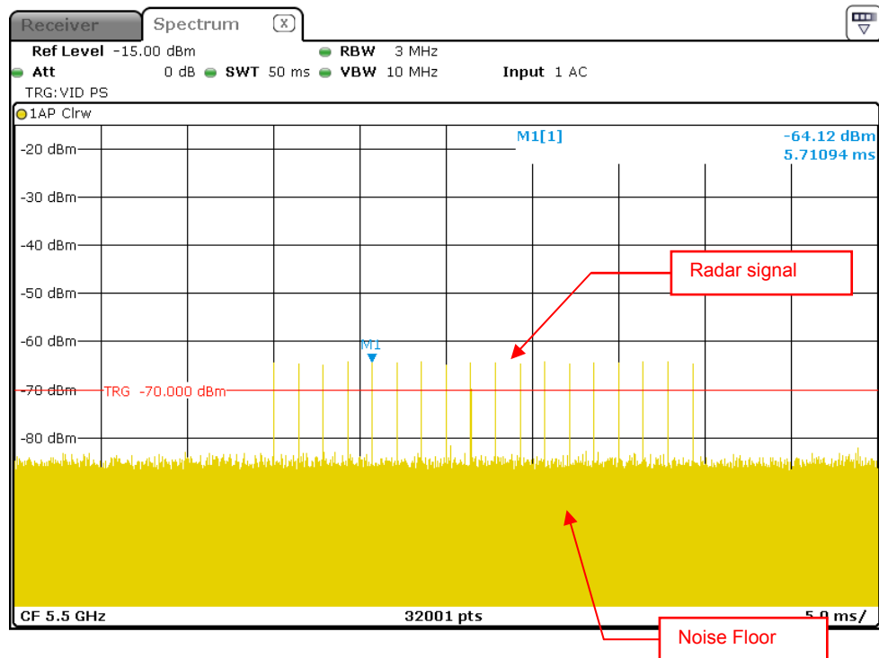
Radar Signal 0
