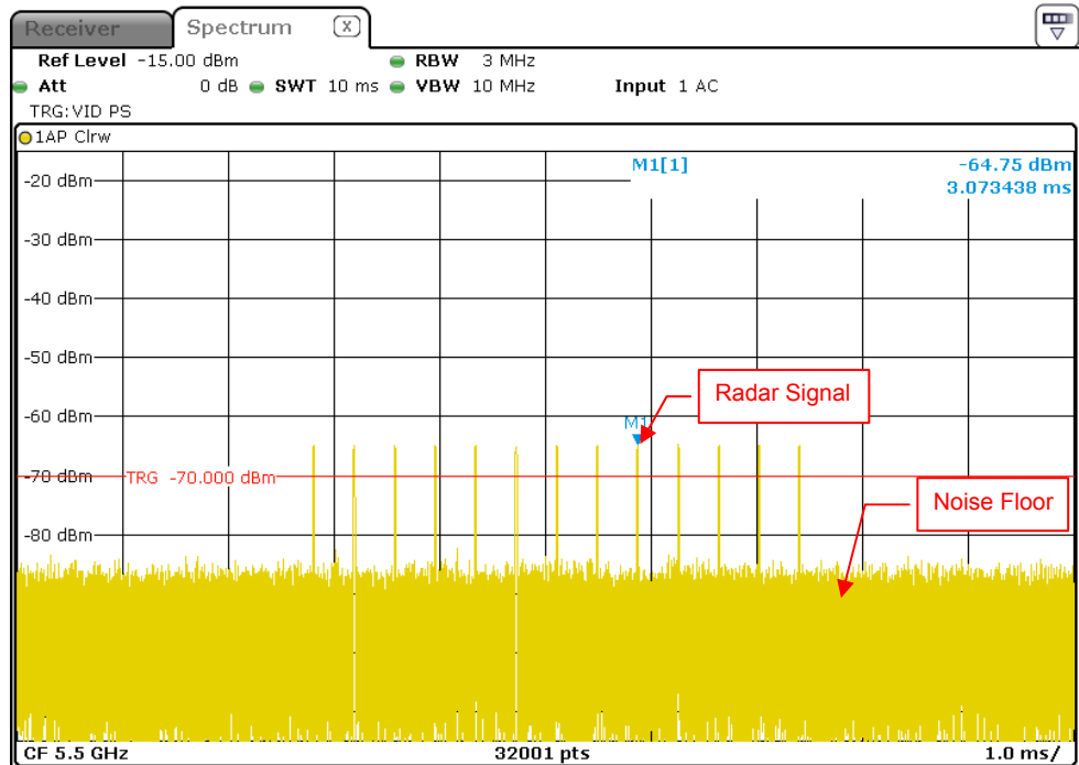
Single Burst of Radar Signal 4
