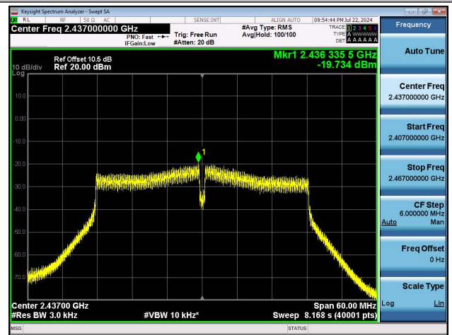
11N40MIMO-Ant1-2437-PASS
