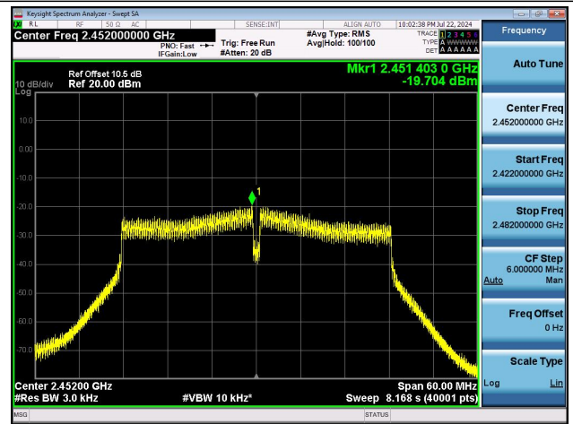
11N40MIMO-Ant1-2452-PASS
