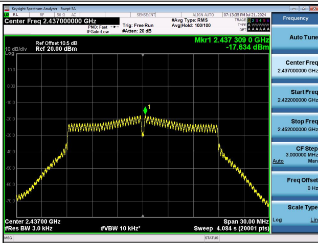
11N20MIMO-Ant0-2437-PASS
