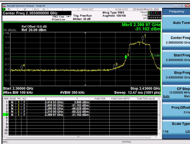
11N20MIMO-Ant0-2412-PASS
