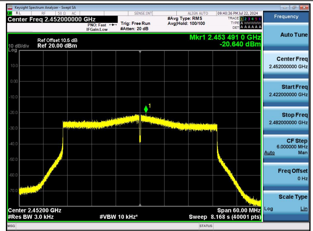
11AX40MIMO-Ant1-2452-PASS
