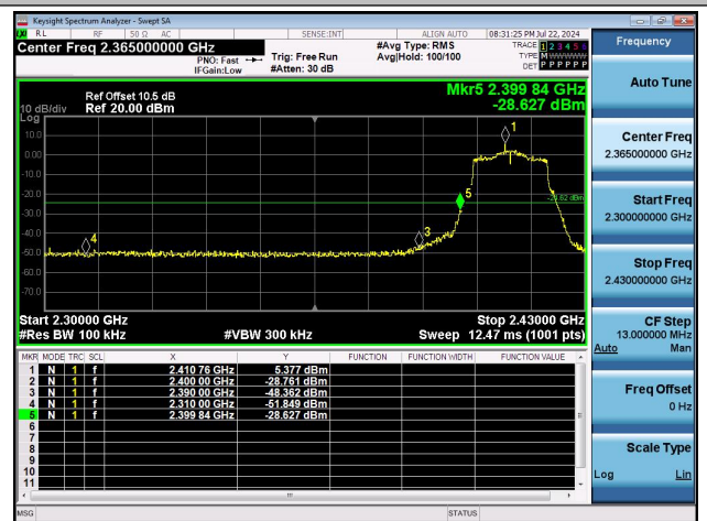
11N20MIMO-Ant1-2412-PASS
