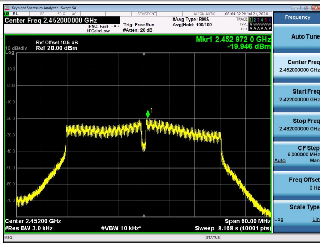
11N40MIMO-Ant0-2452-PASS
