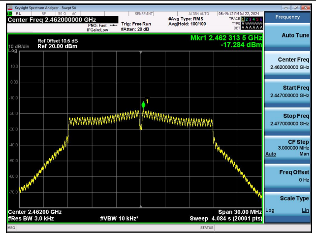
11N20MIMO-Ant1-2462-PASS
