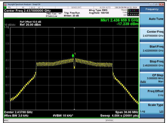
11N20MIMO-Ant1-2437-PASS
