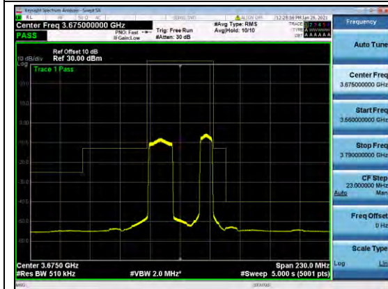
B48-NON-20-15-MASK-L-Q16
