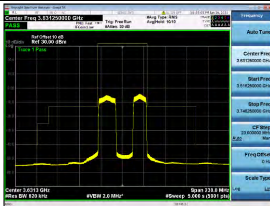
B48-NON-20-15-MASK-H-QPSK
