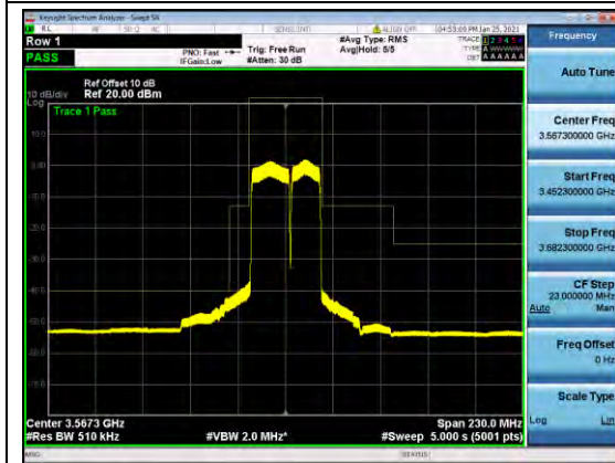
B48-20-15-MASK-M-QPSK
