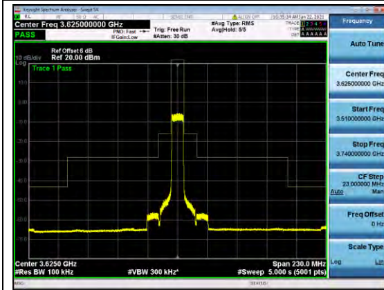
B48-10M-MASK-M-Q64
