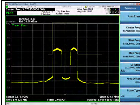
B48-NON-20-15-MASK-M-QPSK
