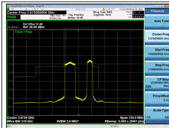
B48-NON-20-10-MASK-H-Q64
