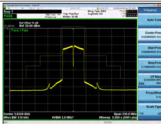
B48-20-20-MASK-M-Q64
