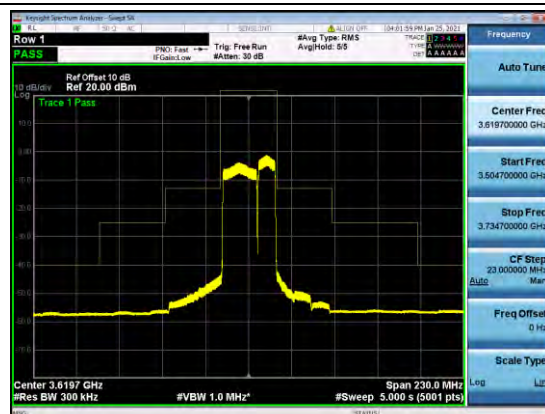
B48-20-10-MASK-M-Q64
