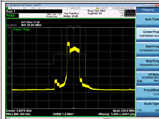
B48-5-20-MASK-H-Q64
