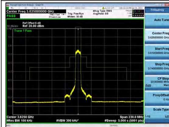
B48-10M-MASK-M-Q64
