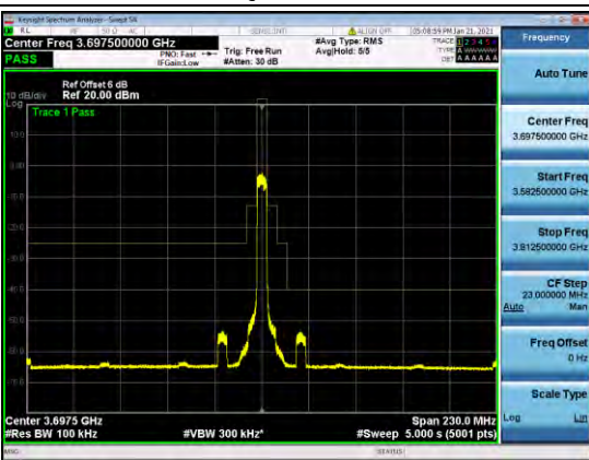
B48-5M-MASK-H-Q64
