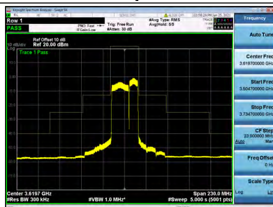
B48-20-10-MASK-H-Q16
