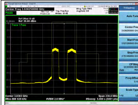
B48-NON-15-20-MASK-H-Q16
