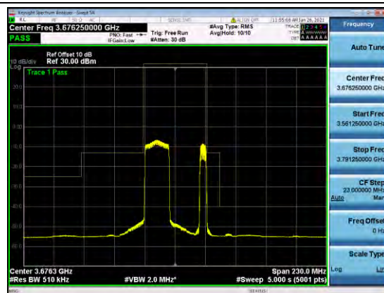
B48-NON-5-20-MASK-L-Q16
