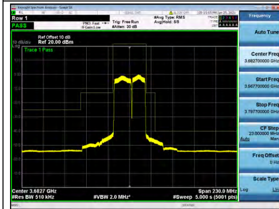
B48-20-20-MASK-L-QPSK
