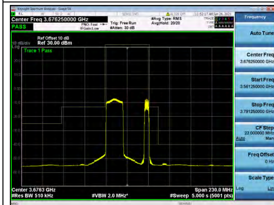
B48-NON-5-20-MASK-L-QPSK
