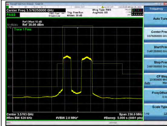
B48-NON-15-20-MASK-M-QPSK
