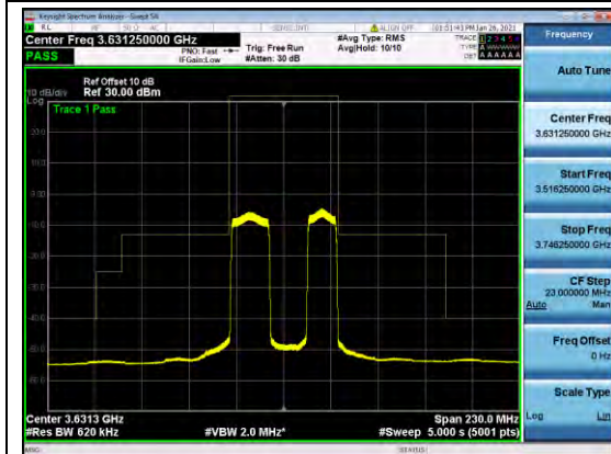
B48-NON-20-15-MASK-M-Q64
