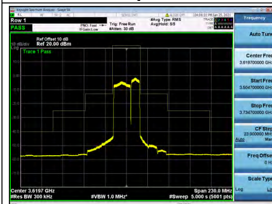
B48-20-10-MASK-H-QPSK
