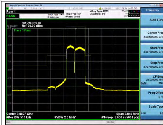
B48-20-10-MASK-L-QPSK
