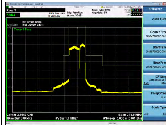
B48-20-10-MASK-L-Q64
