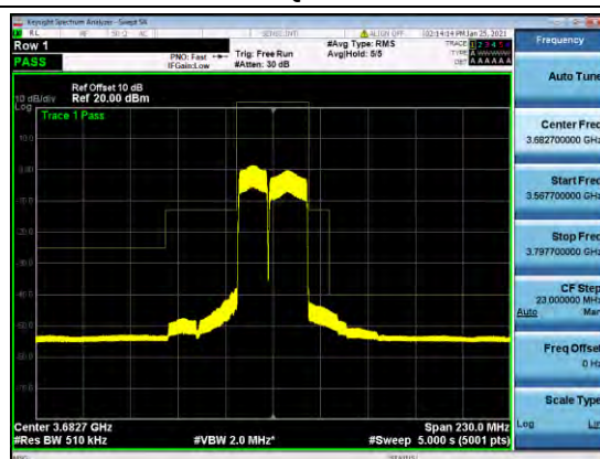
B48-15-20-MASK-H-Q64
