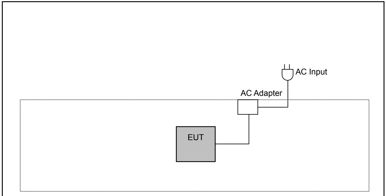
Radiated Emission
