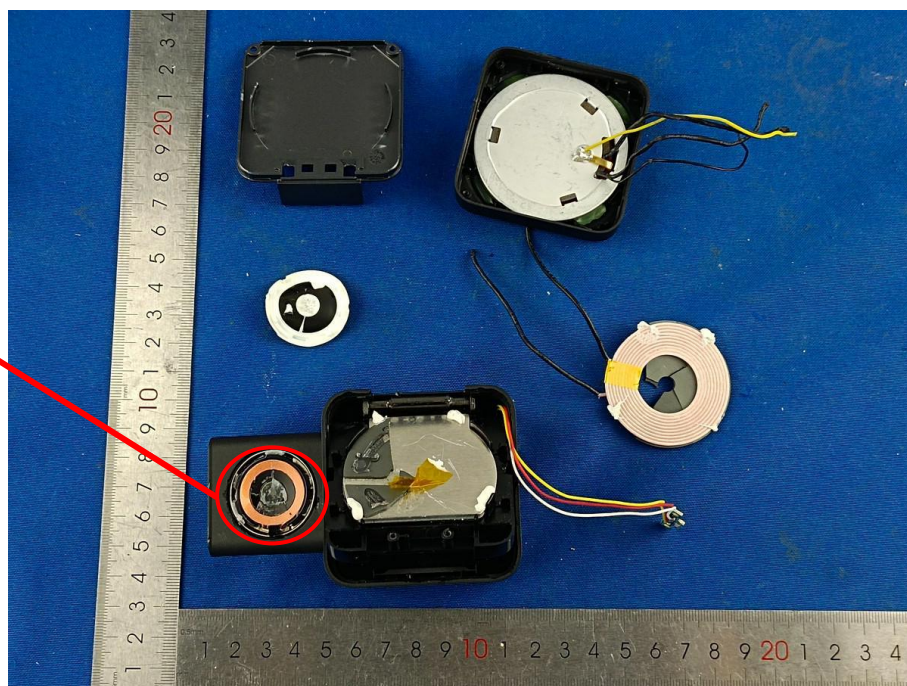
Coil 3
