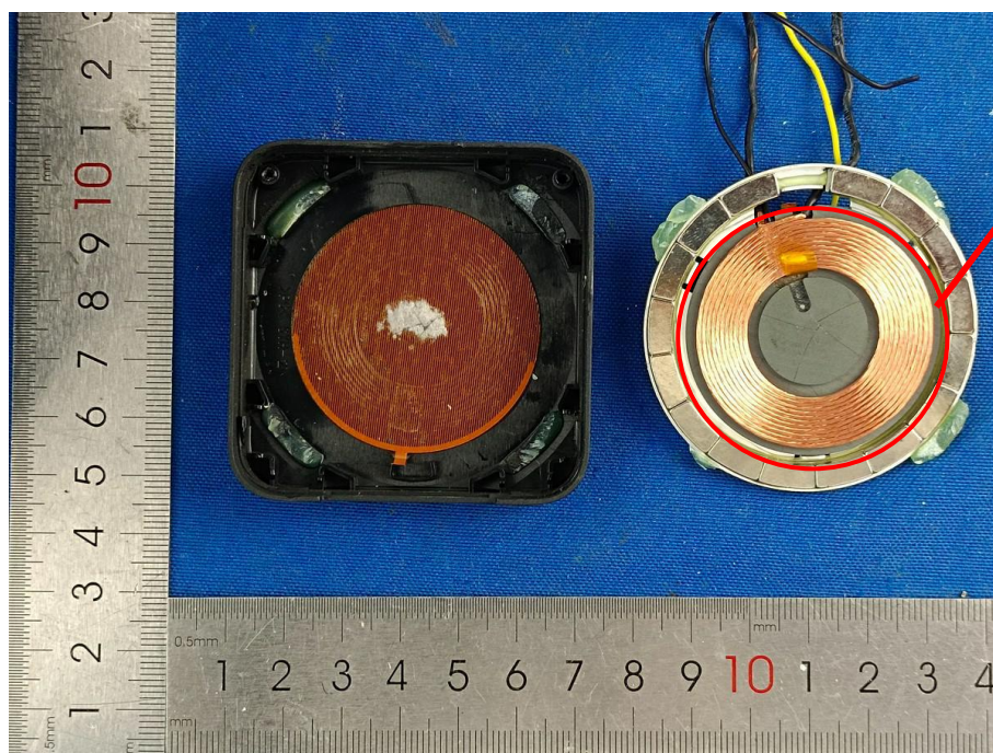
Coil 1
