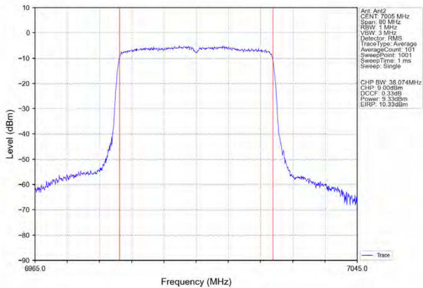
802.11ax(HEW40) MCH 7005MHz RU484 Left Ant2 NTVN
