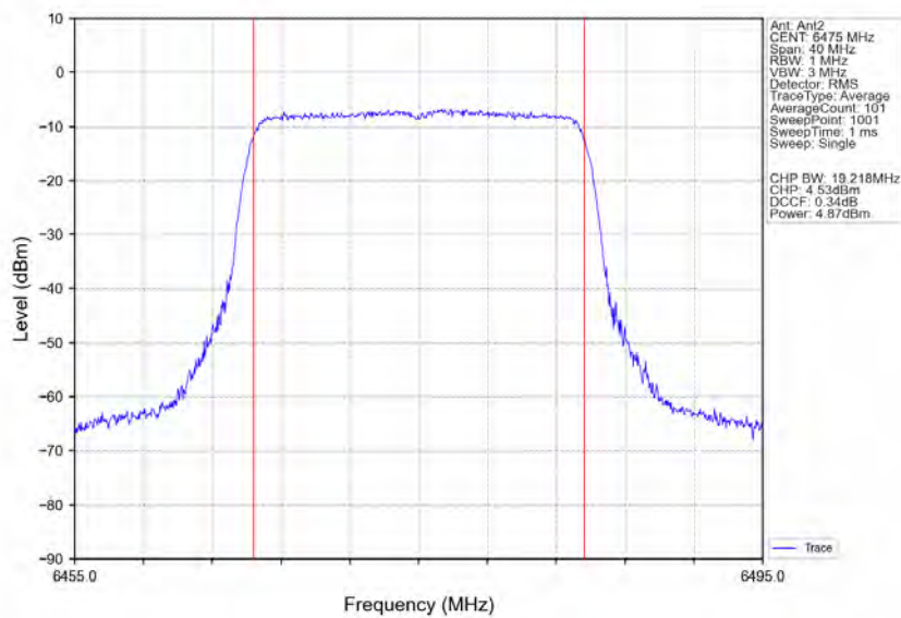
802.11ax(HEW20) MCH 6475MHz RU242 Left Ant2 NTVN
