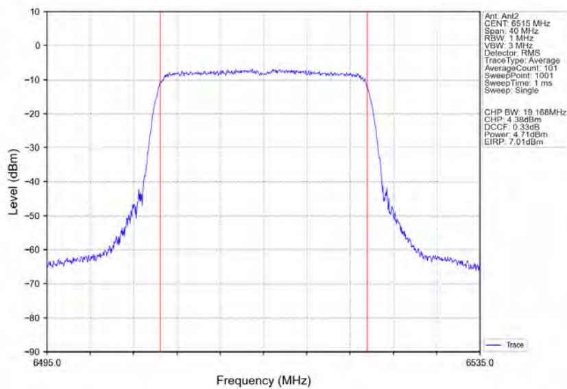
802.11ax(HEW20) HCH 6515MHz RU242 Left Ant2 NTVN
