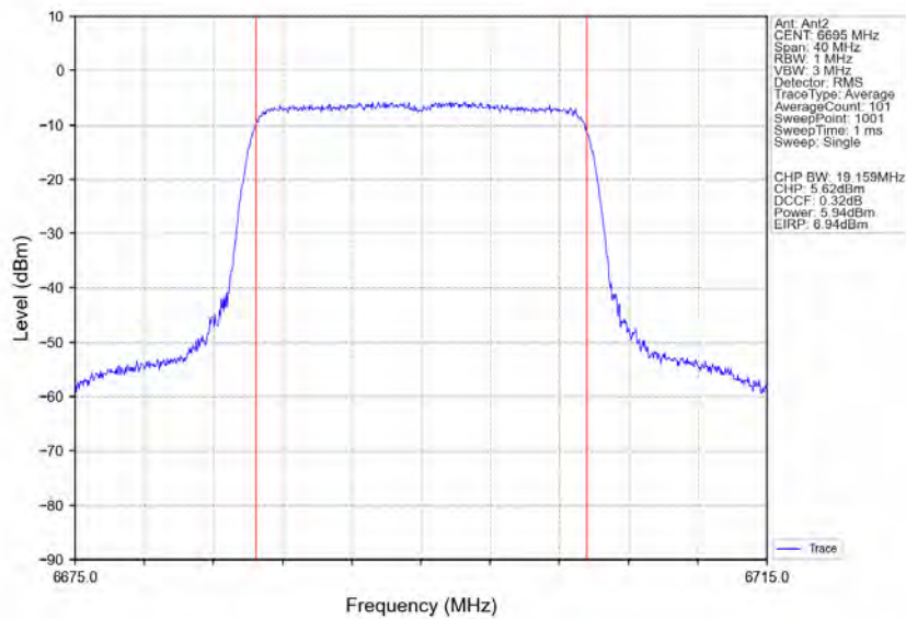
802.11ax(HEW20)_MCH_6695MHz_RU242_Left_Ant2_NTNV
