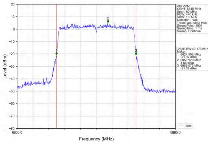
802.11ax(HEW40) HCH 6845MHz RU484 Left Ant2 NTVN
