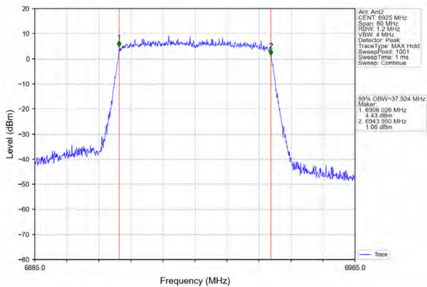
802.11ax(HEW40) LCH_6925MHz RU484 Left_Ant2 NTN
