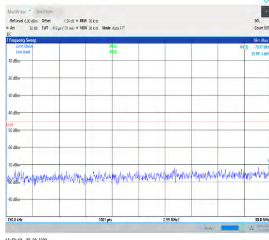
1-N38-PC3-30-40-H-1-DFT-PI2BPSK-Inner_1RB_L ef t-1@1-0.15-30-Ant5-29.79--70.97--45-PASS
