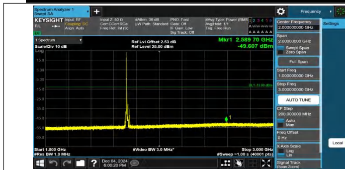
Band4-15MHz-QPSK-20025-1RB#0-1000~3000-PASS
