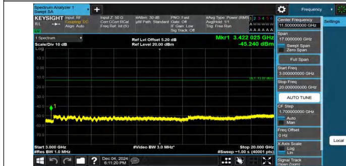
Band4-20MHz-QPSK-20050-1RB#0-3000~20000-PASS
