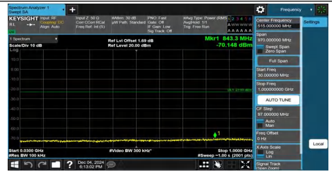
Band4-20MHz-QPSK-20175-1RB#0-30~1000-PASS
