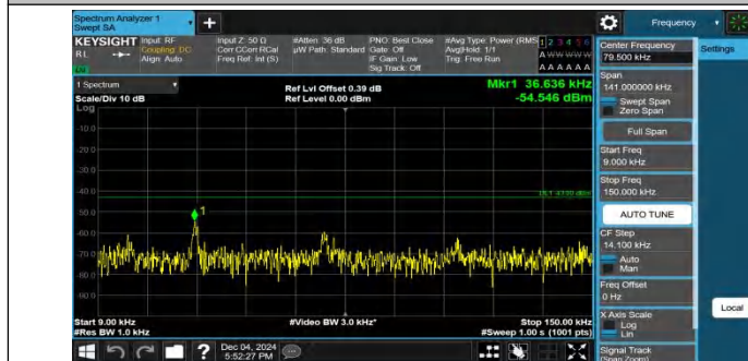
Band4-10MHz-QPSK-20350-1RB#0-0.009~0.15-PASS
