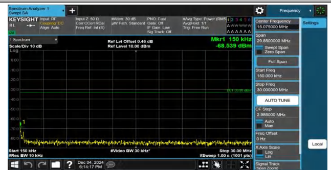
Band4-20MHz-QPSK-20175-100RB#0-0.15~30-PASS
