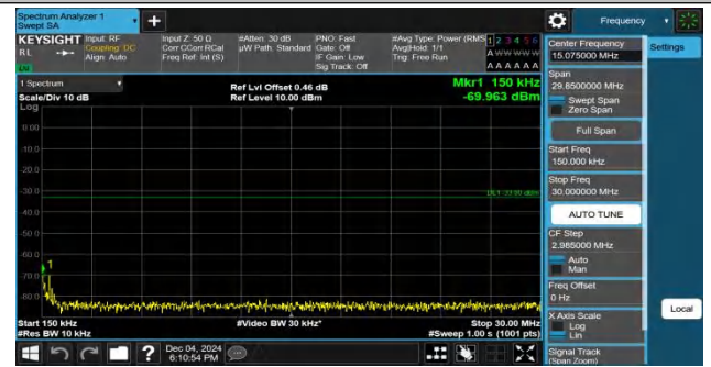
Band4-20MHz-QPSK-20050-1RB#0-0.15~30-PASS
