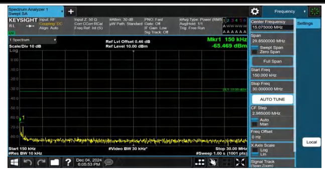
Band4-15MHz-QPSK-20325-75RB#0-0.15~30-PASS
