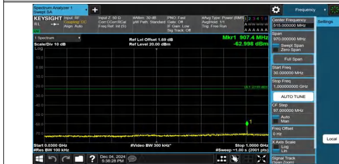
Band4-5MHz-QPSK-20175-1RB#0-30~1000-PASS
