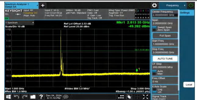
Band4-20MHz-QPSK-20050-1RB#0-1000~3000-PASS
