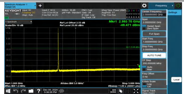
Band4-5MHz-QPSK-20175-1RB#0-1000~3000-PASS
