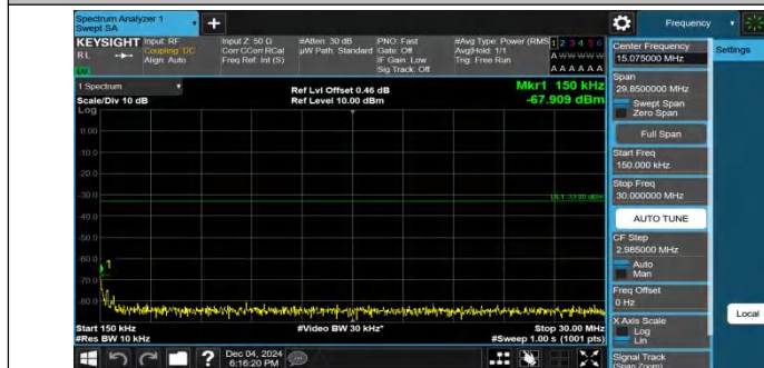
Band4-20MHz-QPSK-20300-100RB#0-0.15~30-PASS
