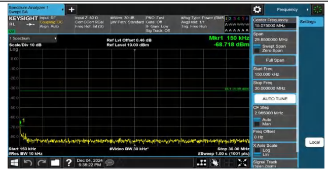
Band4-5MHz-QPSK-20175-1RB#0.15~30-PASS
