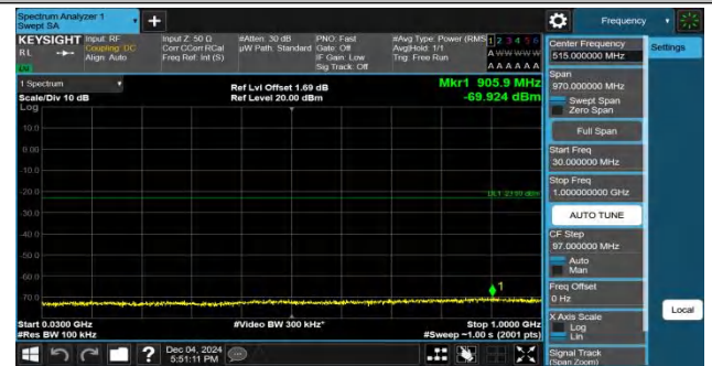
Band4-10MHz-QPSK-20175-1RB#49-30~1000-PASS
