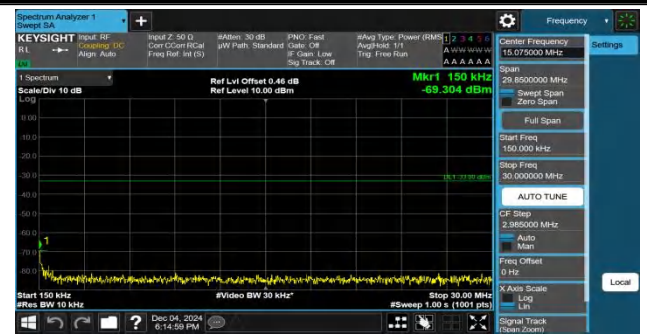
Band4-20MHz-QPSK-20300-1RB#0-0.15~30-PASS
