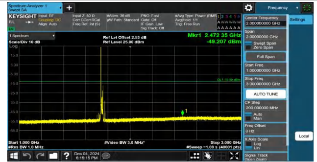
Band4-20MHz-QPSK-20300-1RB#0-1000~3000-PASS
