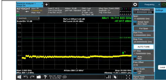
Band4-20MHz-QPSK-20175-100RB#0-3000~20000-PASS
