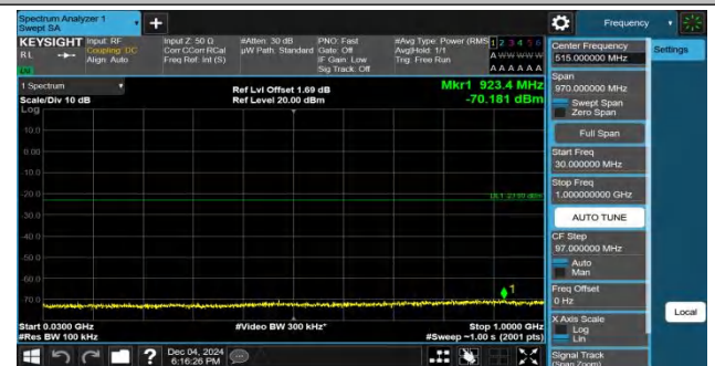
Band4-20MHz-QPSK-20300-100RB#0-30~1000-PASS
