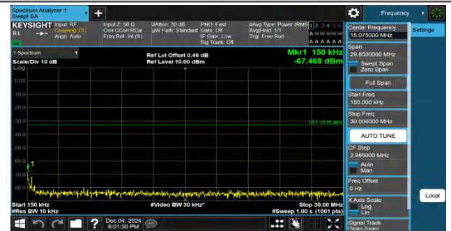
Band4-15MHz-QPSK-20025-75RB#0-0.15~30-PASS
