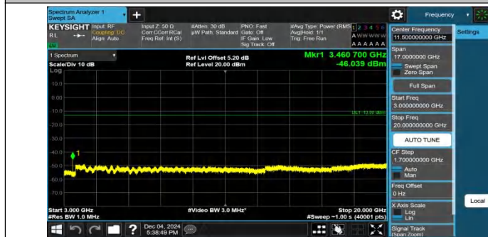
Band4-5MHz-QPSK-20175-1RB#0-3000~20000-PASS
