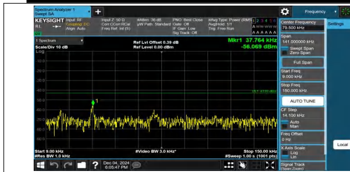
Band4-15MHz-QPSK-20325-75RB#0-0.009~0.15-PASS
