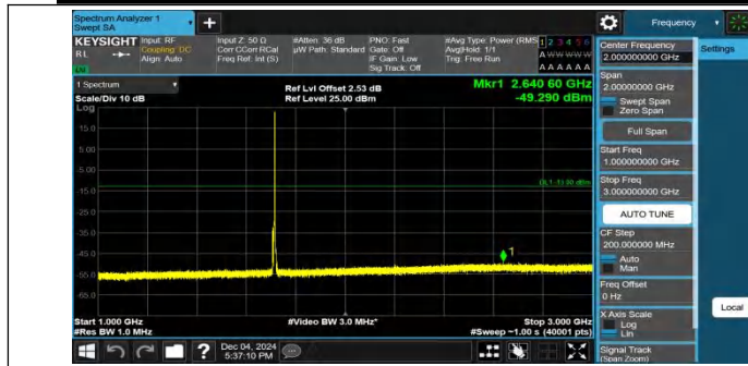
Band4-5MHz-QPSK-19975-1RB#24-1000~3000-PASS
