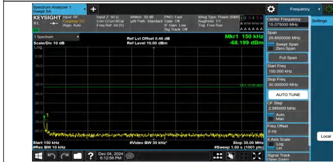
Band4-20MHz-QPSK-20175-1RB#0-0.15~30-PASS
