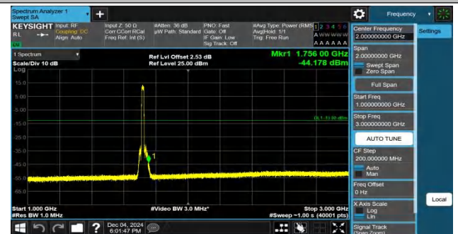
Band4-15MHz-QPSK-20025-75RB#0-1000~3000-PASS
