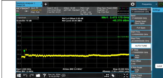
Band4-20MHz-QPSK-20300-1RB#0-3000~20000-PASS
