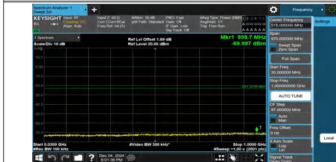
Band4-15MHz-QPSK-20025-75RB#0-30~1000-PASS
