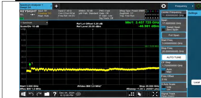
Band4-20MHz-QPSK-20050-1RB#99-3000~20000-PASS
