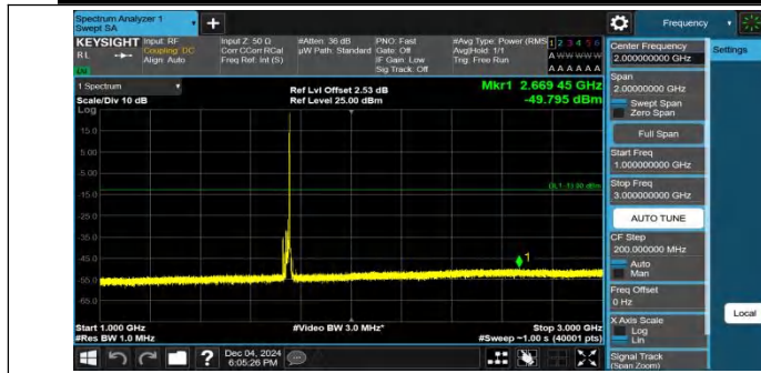
Band4-15MHz-QPSK-20325-1RB#74-1000~3000-PASS
