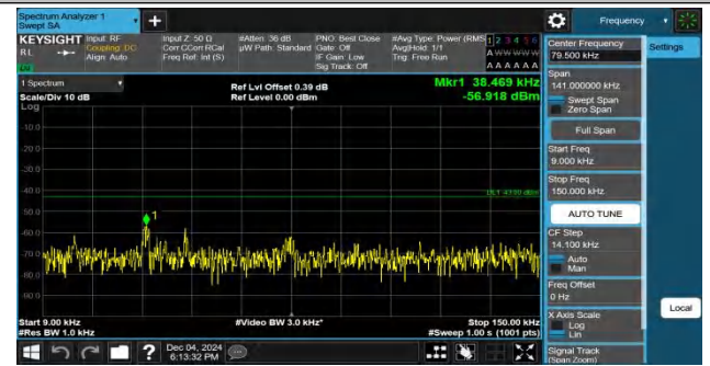
Band4-20MHz-QPSK-20175-1RB#99-0.009~0.15-PASS
