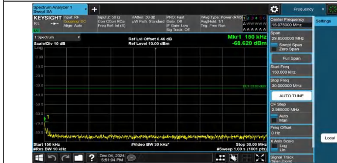
Band4-10MHz-QPSK-20175-1RB#49-0.15~30-PASS
