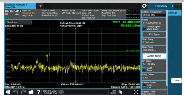
Band4-5MHz-QPSK-20175-25RB#0-0.009~0.15-PASS
