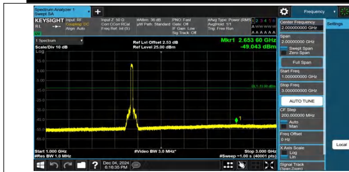
Band4-20MHz-QPSK-20300-100RB#0-1000~3000-PASS
