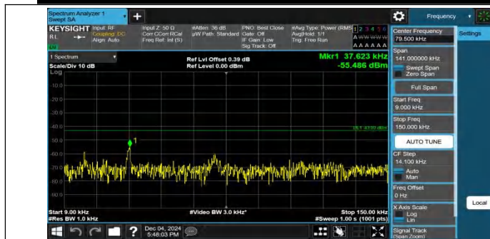
Band4-10MHz-QPSK-20000-1RB#0-0.009~0.15-PASS
