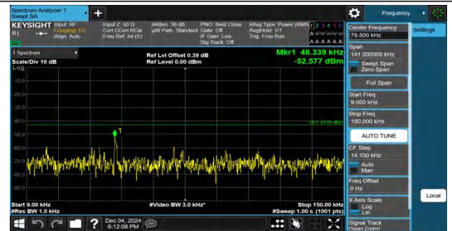
Band4-20MHz-QPSK-20050-100RB#0-0.009~0.15-PASS
