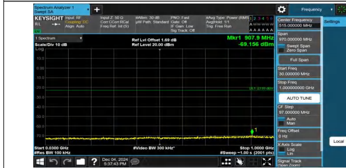
Band4-5MHz-QPSK-19975-25RB#0-30~1000-PASS
