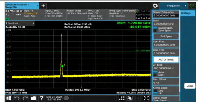
Band4-5MHz-QPSK-19975-25RB#0-1000~3000-PASS
