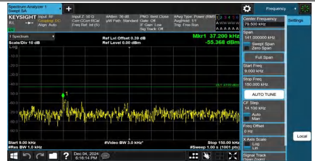
Band4-20MHz-QPSK-20300-100RB#0-0.009~0.15-PASS
