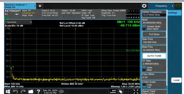
Band4-10MHz-QPSK-20350-1RB#0-0.15~30-PASS
