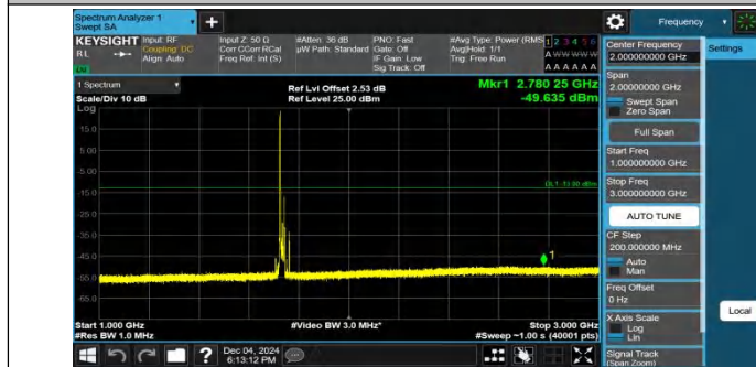
Band4-20MHz-QPSK-20175-1RB#0-1000~3000-PASS
