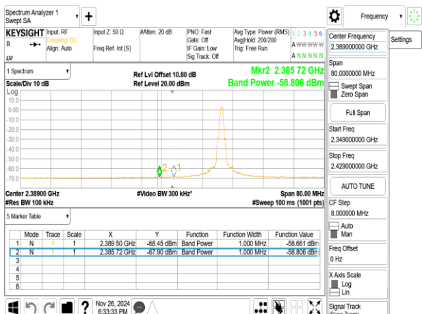
CBE_BLE_500K_2402MHz
