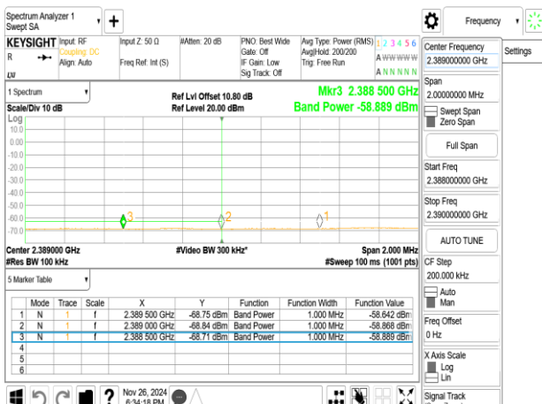
CBE_BLE_500K_2402MHz
