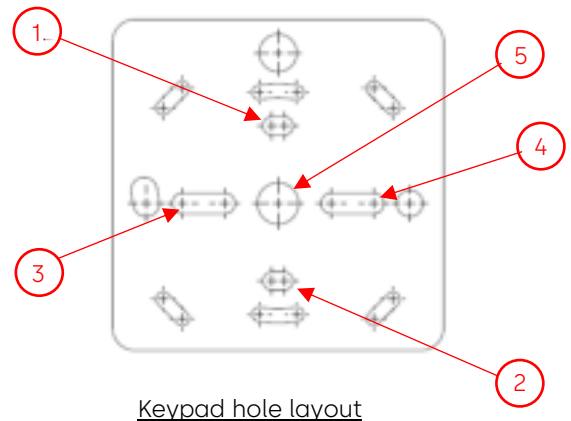
Keypad hole layout
