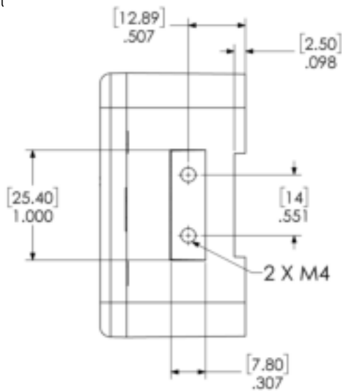
Lock (Profile View)
