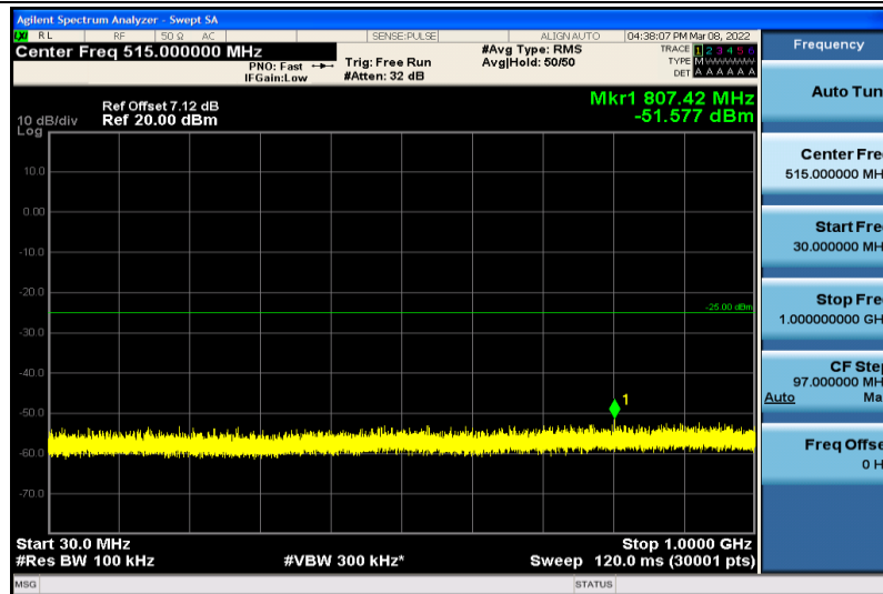
Band7-15MHz-64QAM-20825-1RB#0-30~1000MHz
