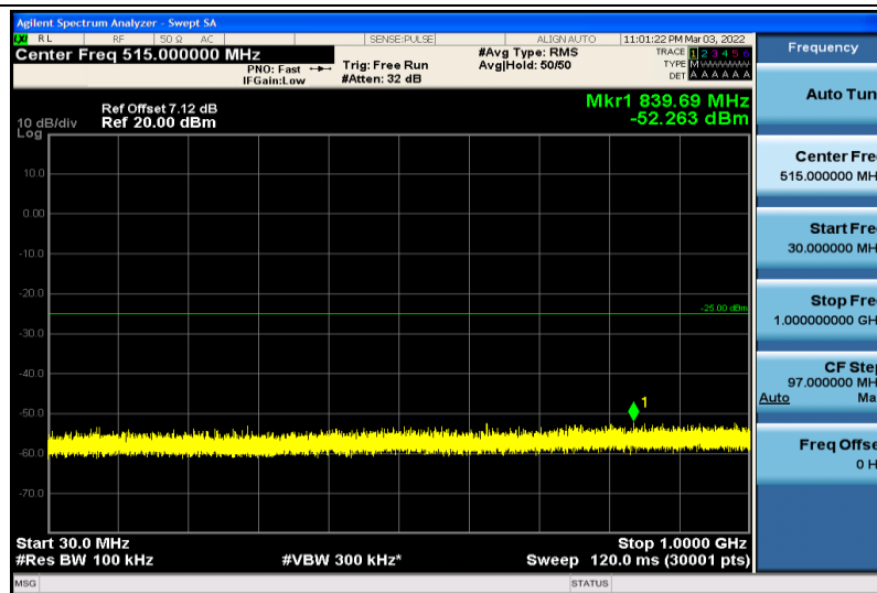
Band7-5MHz-16QAM-20775-1RB#0-30~1000MHz
