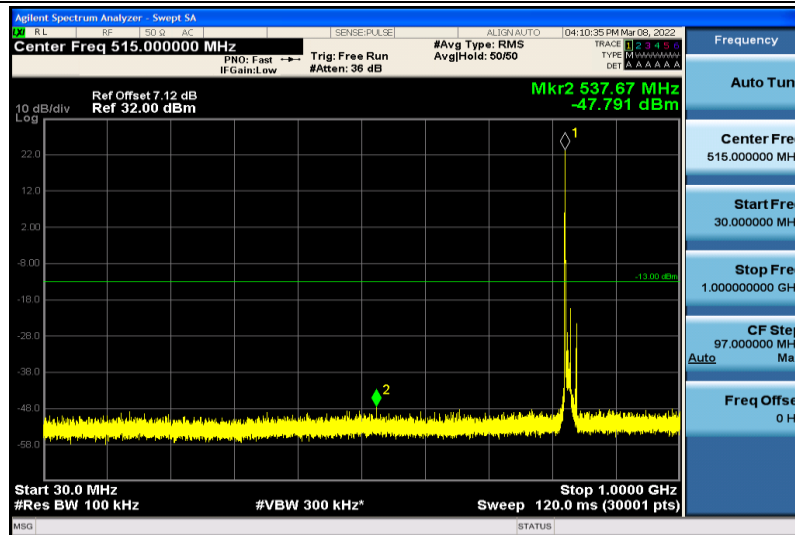
Band5-10MHz-64QAM-20450-1RB#0-30~1000MHz
