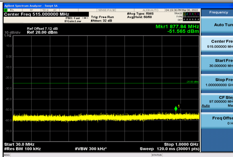
Band7-5MHz-64QAM-21425-1RB#0-30~1000MHz
