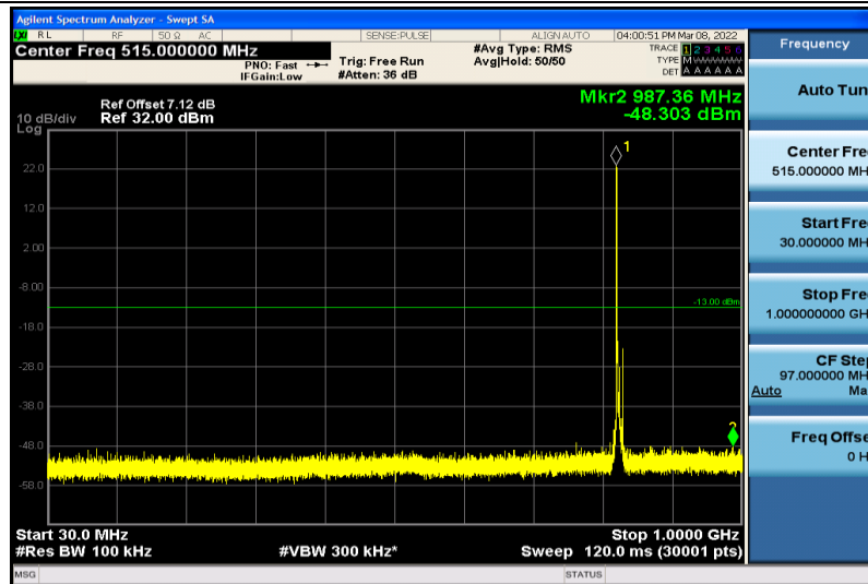
Band5-5MHz-64QAM-20425-1RB#0-30~1000MHz
