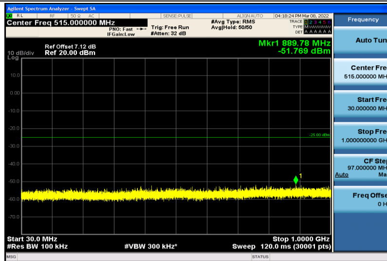
Band7-5MHz-64QAM-20775-1RB#0-30~1000MHz
