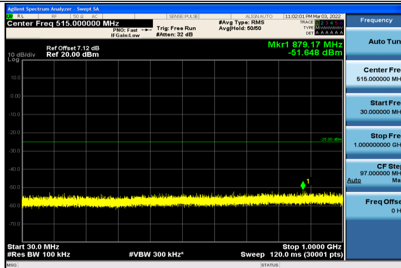
Band7-5MHz-QPSK-21100-1RB#0-30~1000MHz
