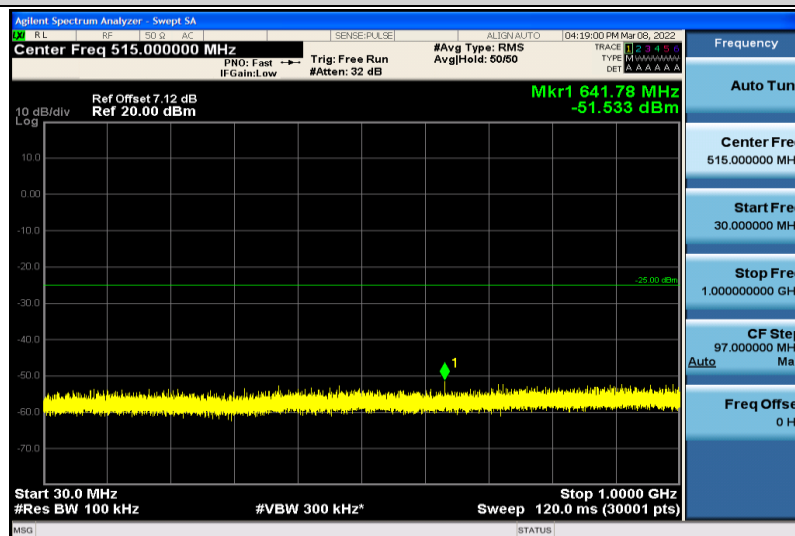
Band7-5MHz-64QAM-21100-1RB#0-30~1000MHz
