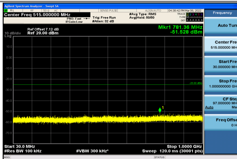
Band7-15MHz-64QAM-21100-1RB#0-30~1000MHz
