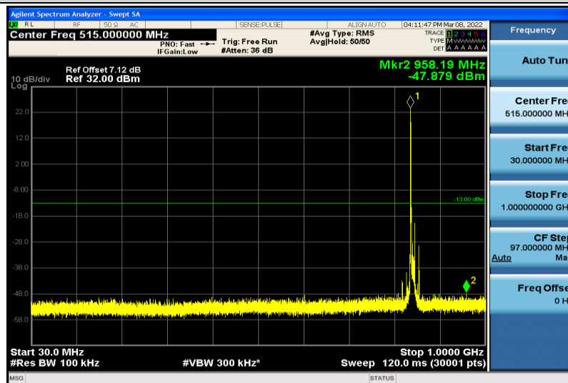
Band5-10MHz-64QAM-20600-1RB#0-30~1000MHz
