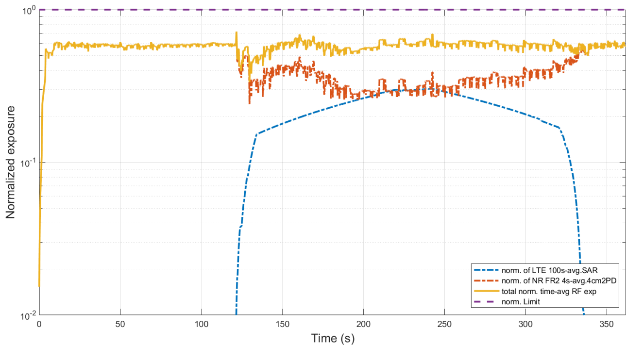
Figure 7.9-2 Total normalized time-average RF exposure in F_TC08
