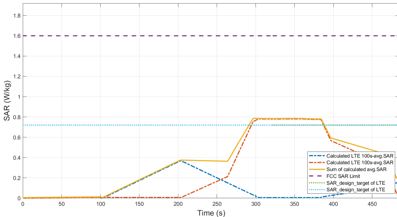
Figure 6.6-4 Total time-averaged SAR
