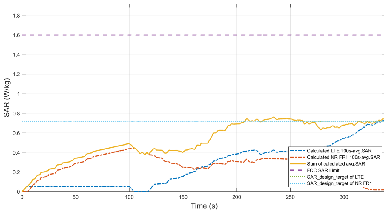
Figure 6.8-2 Total time-averaged SAR
