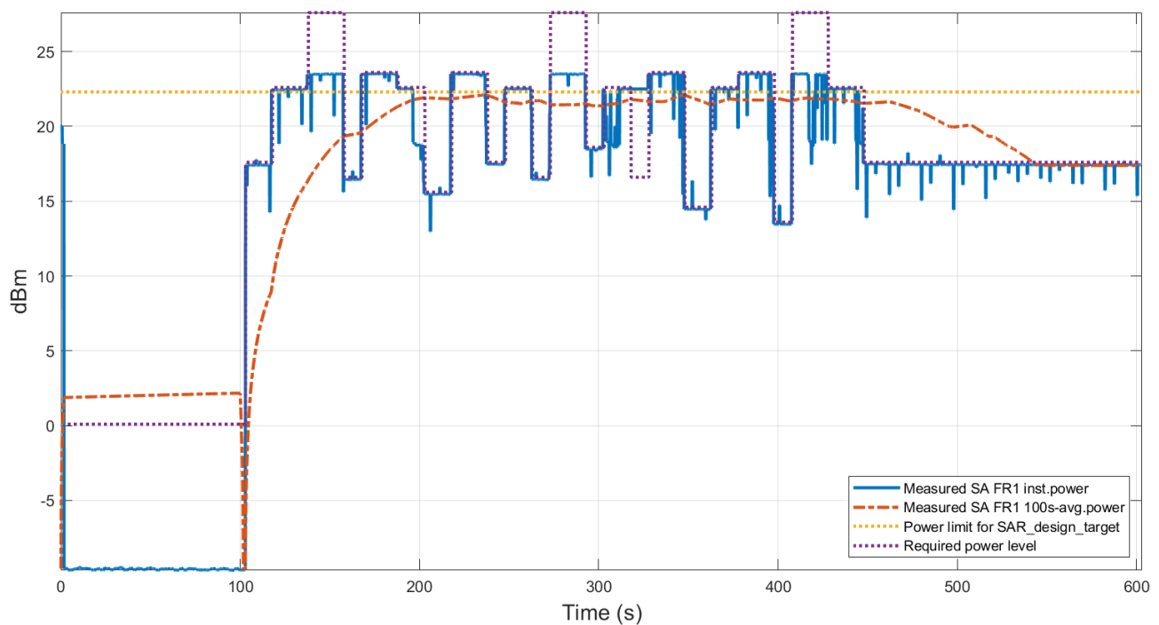
Figure 6.3-15 Conducted Tx power
