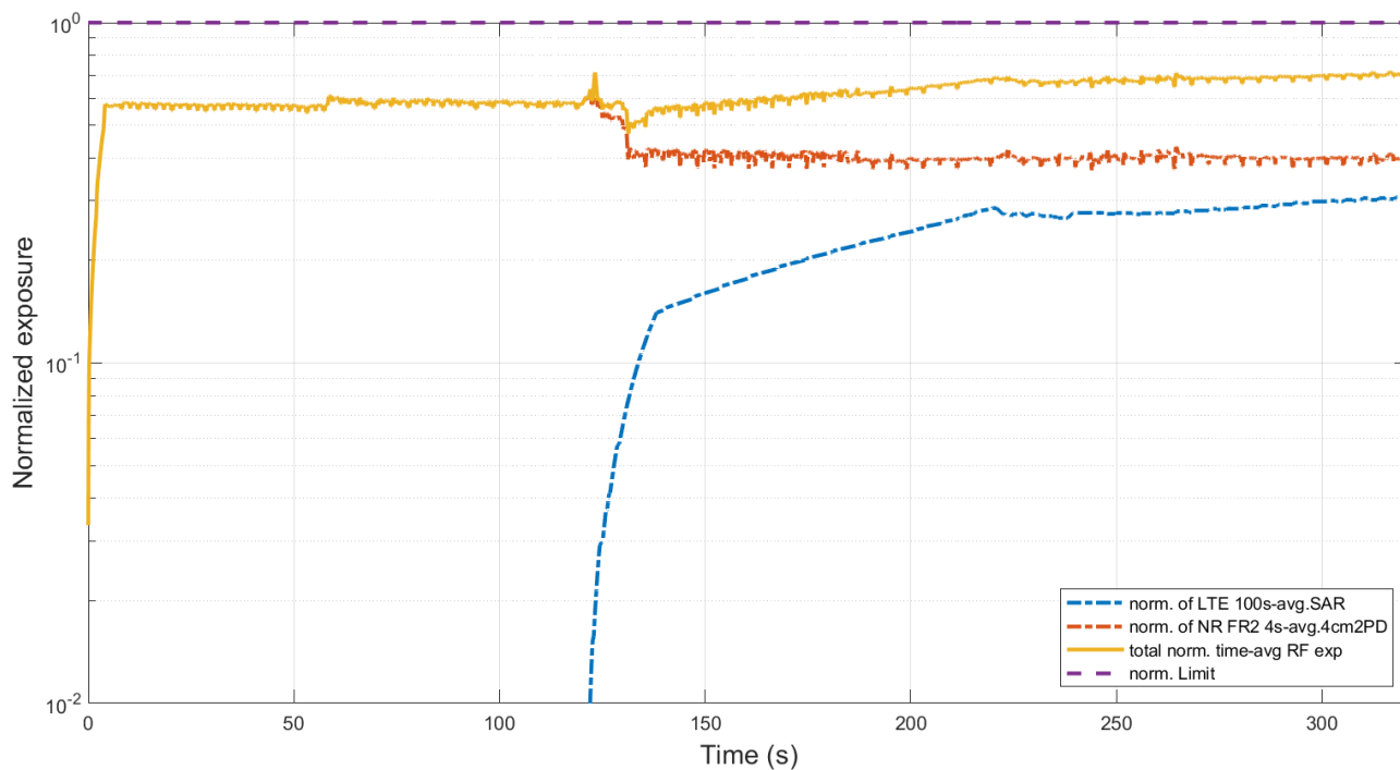
Figure 7.5-2 Total normalized time-average RF exposure in F_TC04
