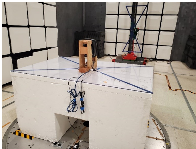
Figure 3 - Radiated emissions above 30 MHz.
