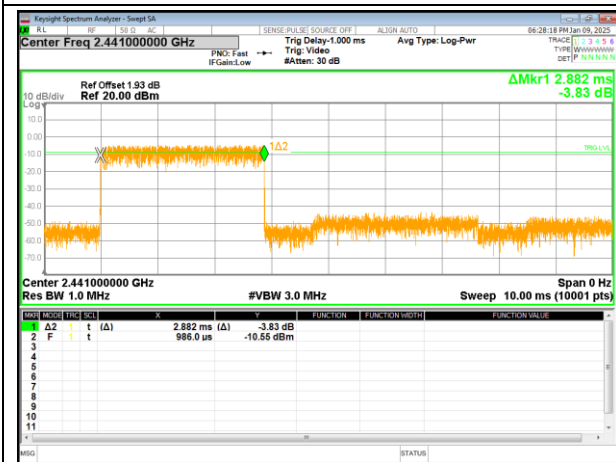
2DH5-2441MHz-One burst
