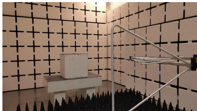
Radiated Emissions for 1GHz~5GHz
