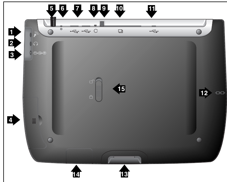
Figure 2: Back of airpanel V150
