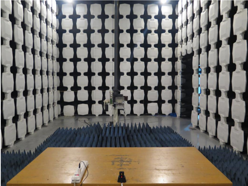
Pic2. Radiated emissions (1GHz-18GHz)
