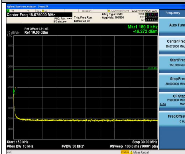
EGPRS850-190-8-0.15~30MHz-PASS
