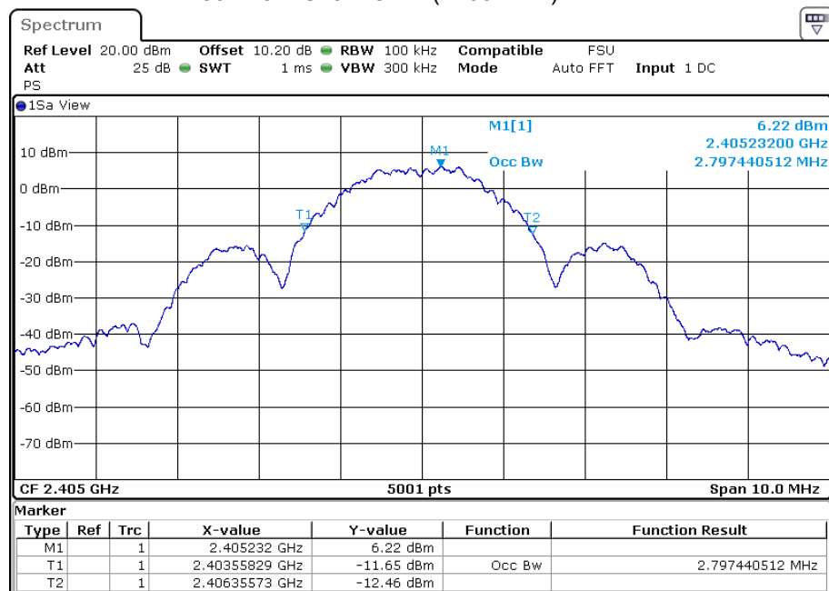
802.15.4 Channel 11 (2405 MHz)
