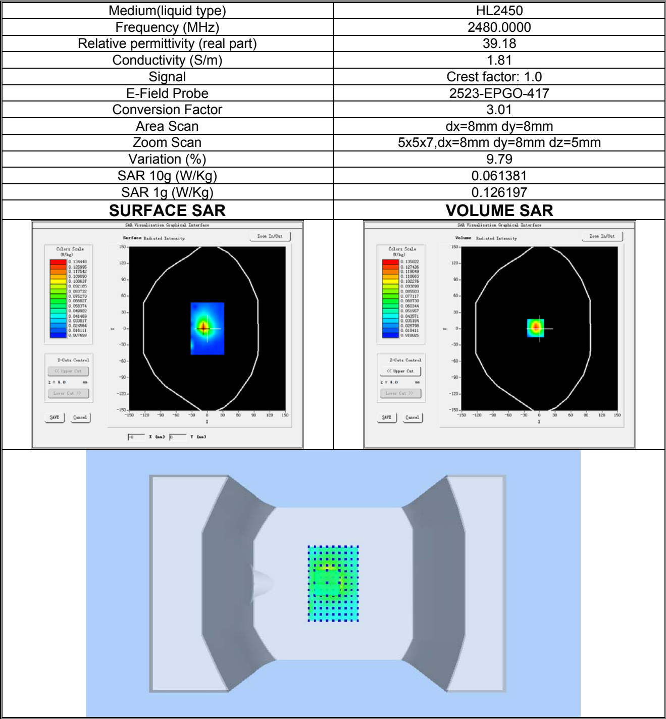
Plot 30: Bluetooth, High channel (Body-worn/ Hotspot, Front Side) Product Description: Smart Phone Test Date: 2024-10-11
