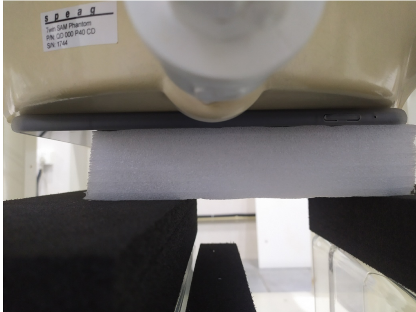
Body (Worn) Back Setup Photo (0mm)
