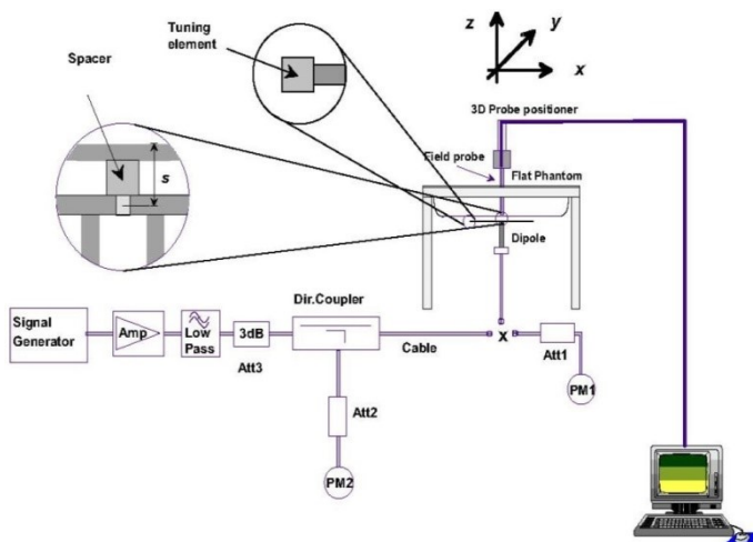
Fig 8.3.1 System Performance Check Setup
