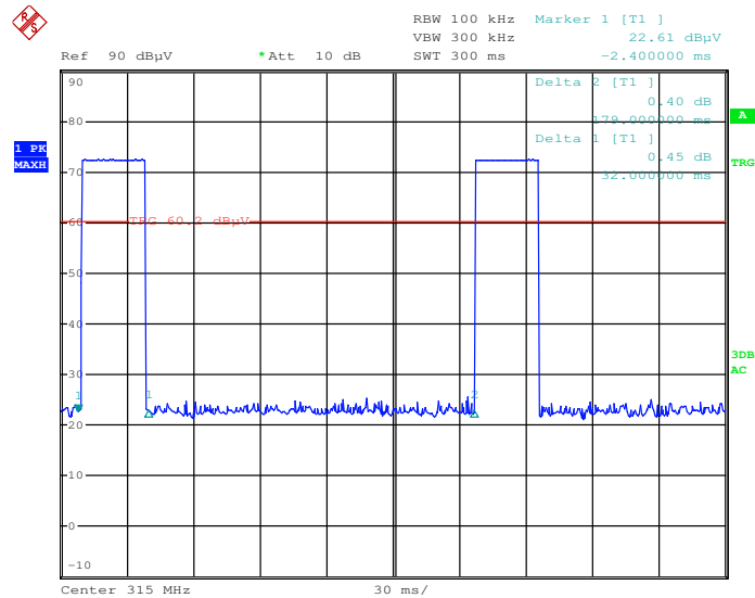
Duty Cycle
