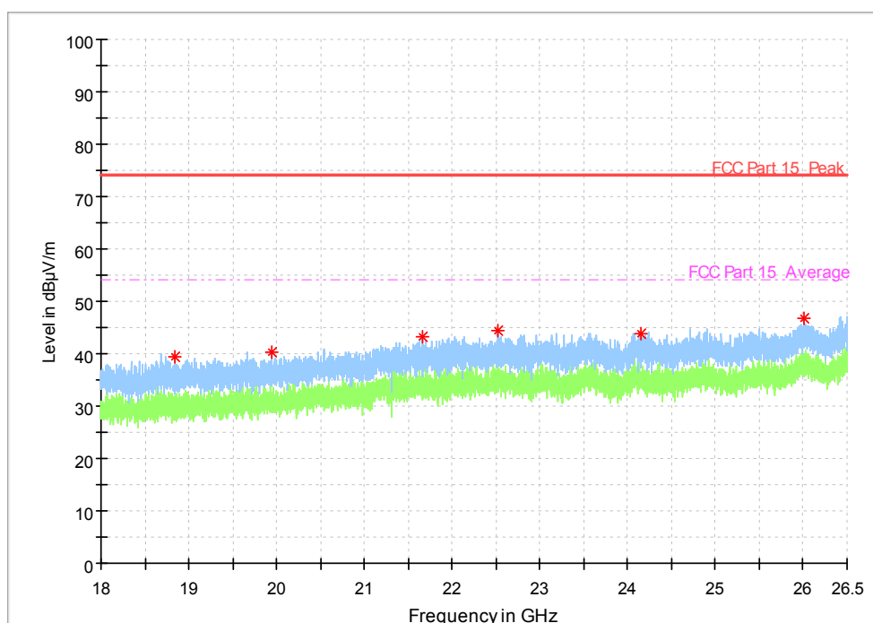
Fig. 37 Radiated Spurious Emission (802.11n-HT20, ch44, 18 GHz-26.5 GHz)
