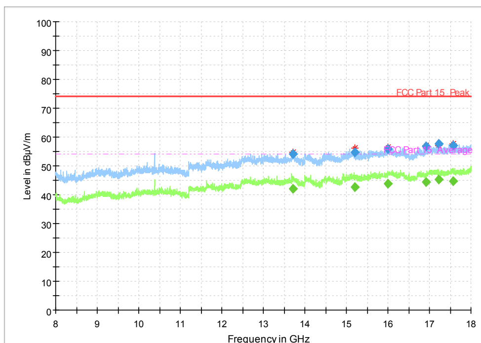
Fig. 41 Radiated Spurious Emission (802.11n-HT40, ch38, 8 GHz-18 GHz)
