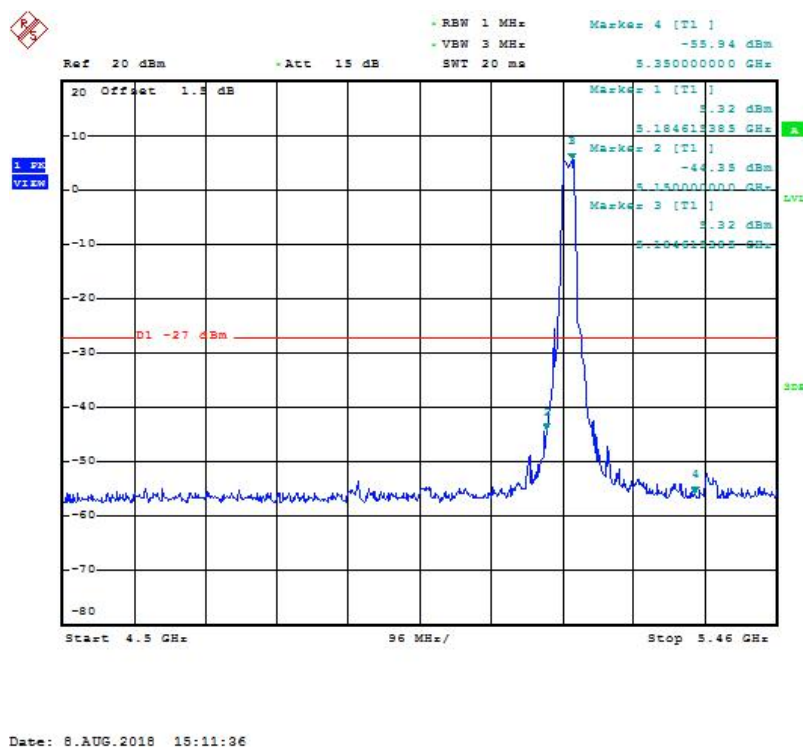
Fig. 17 Band Edges (802.11a, 5180MHz)
