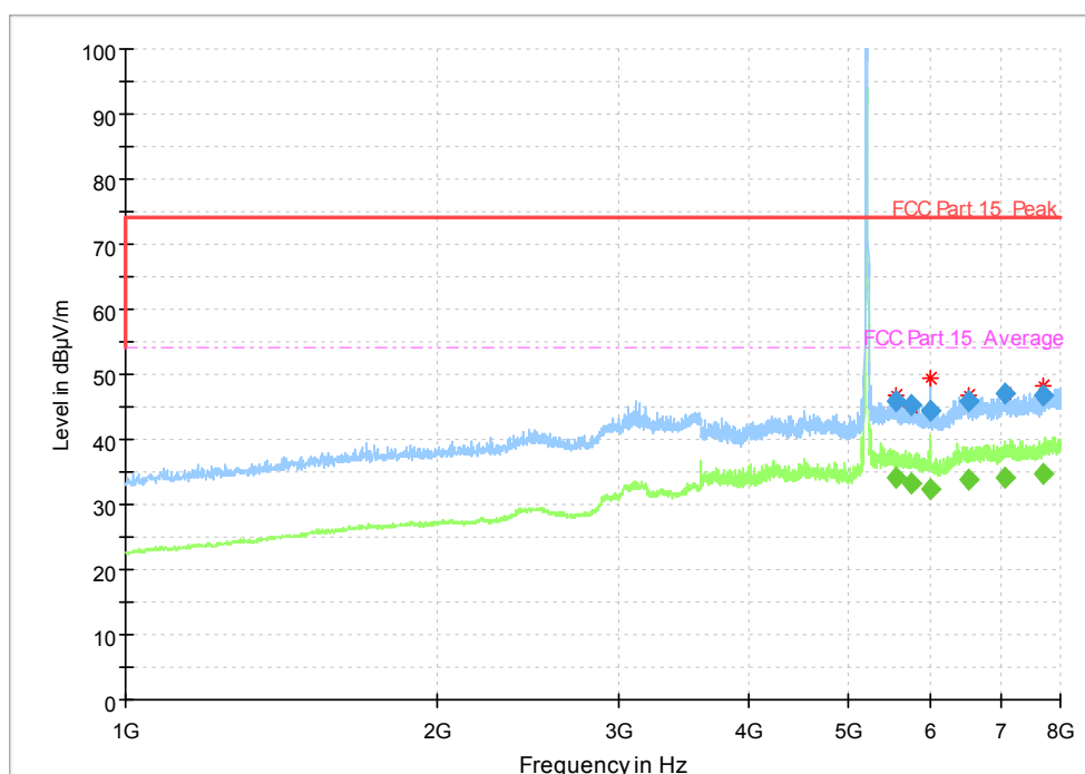
Fig. 35 Radiated Spurious Emission (802.11n-HT20, ch44, 1 GHz-8 GHz)
