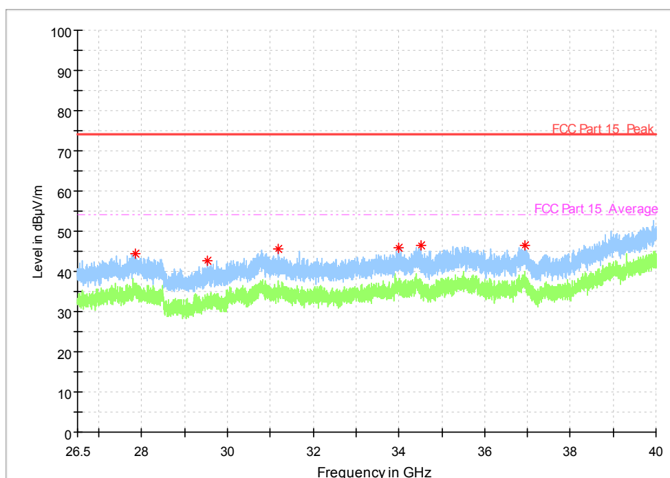
Fig. 43 Radiated Spurious Emission (802.11n-HT40, ch38, 26.5 GHz-40 GHz)
