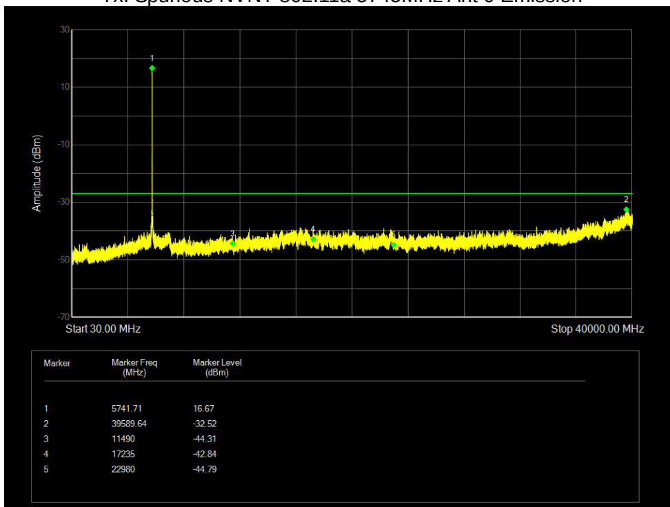
Tx. Spurious NVNT 802.11a 5745MHz Ant 0 Emission
