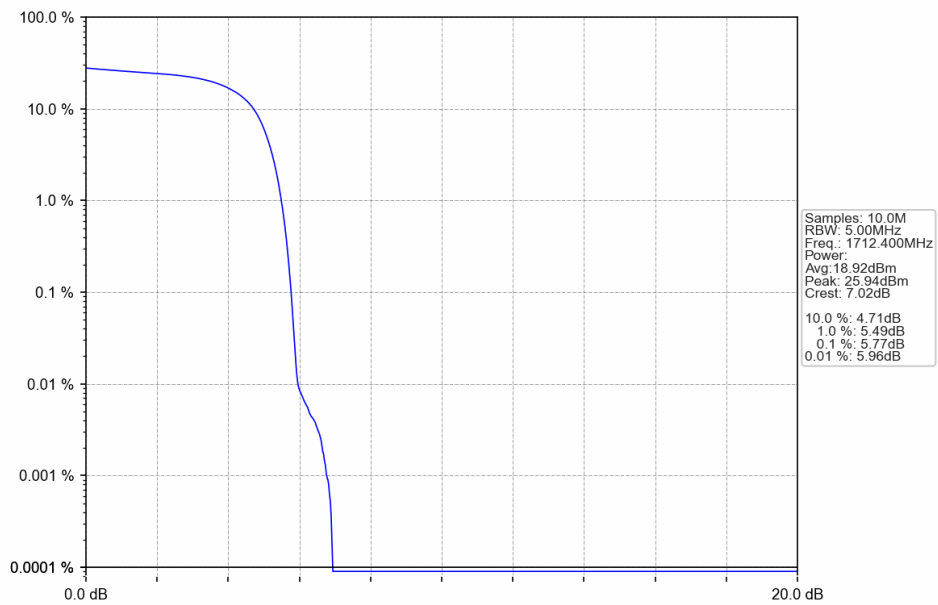
Band4_HSDPA_LCH_1712.4MHz_Subtest 1_NTN
