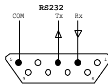
Figure 8-11 : DB9 Connector
