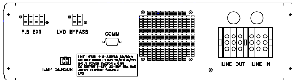
Figure 8-3: BSPS Main Rack - Rear Panel
