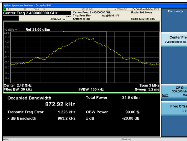
8DPSK 20 dB BW & 99% OBW (Ch. 78)
