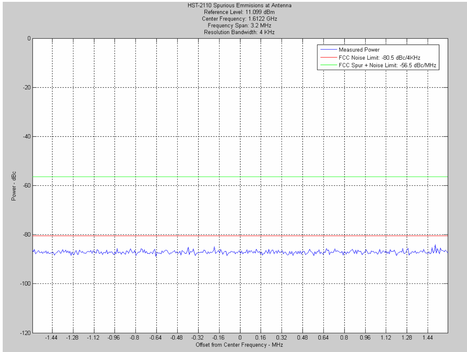
Figure 8 – 1610.6 to 1613.8 MHz
