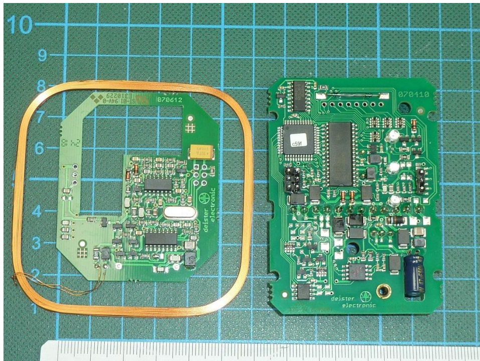
181073eut22: PRD5/2 PCBs view 1
