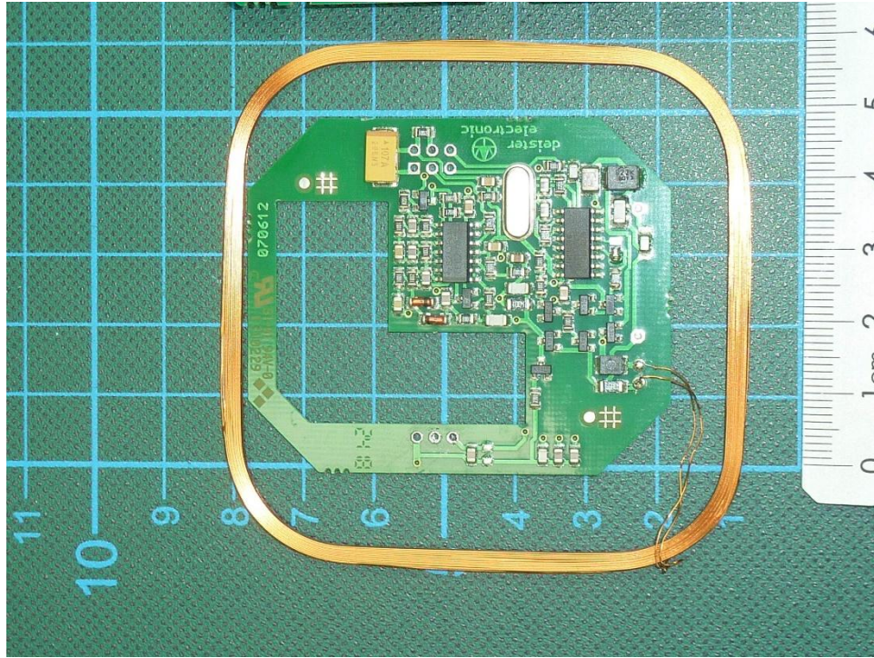
181073eut23: PRD5/2 PCB1 bottom view
