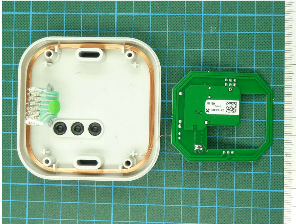
181073eut9.JPG: KPD5/2 inside view 3
