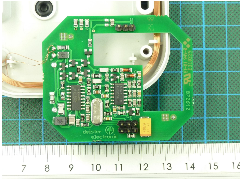
181073eut11.JPG: KPD5/2 PCB 1 top view 1
