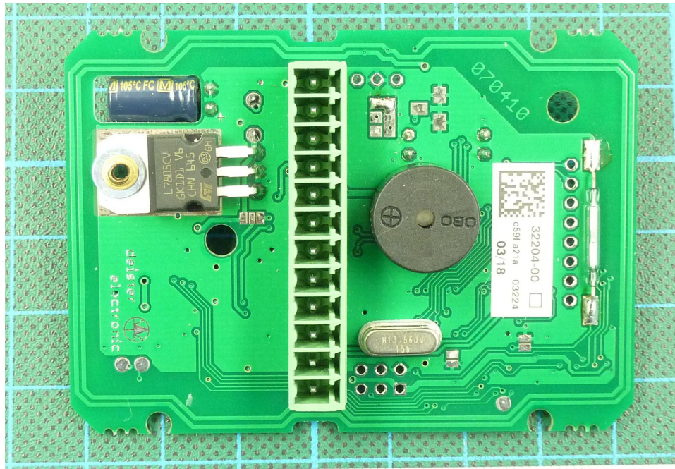
181073eut13.JPG: KPD5/2 PCB 2 bottom view
