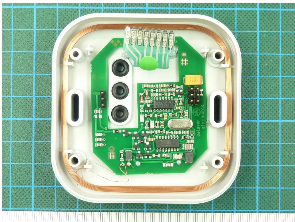
181073eut12.JPG: KPD5/2 PCB 1 top view 2
