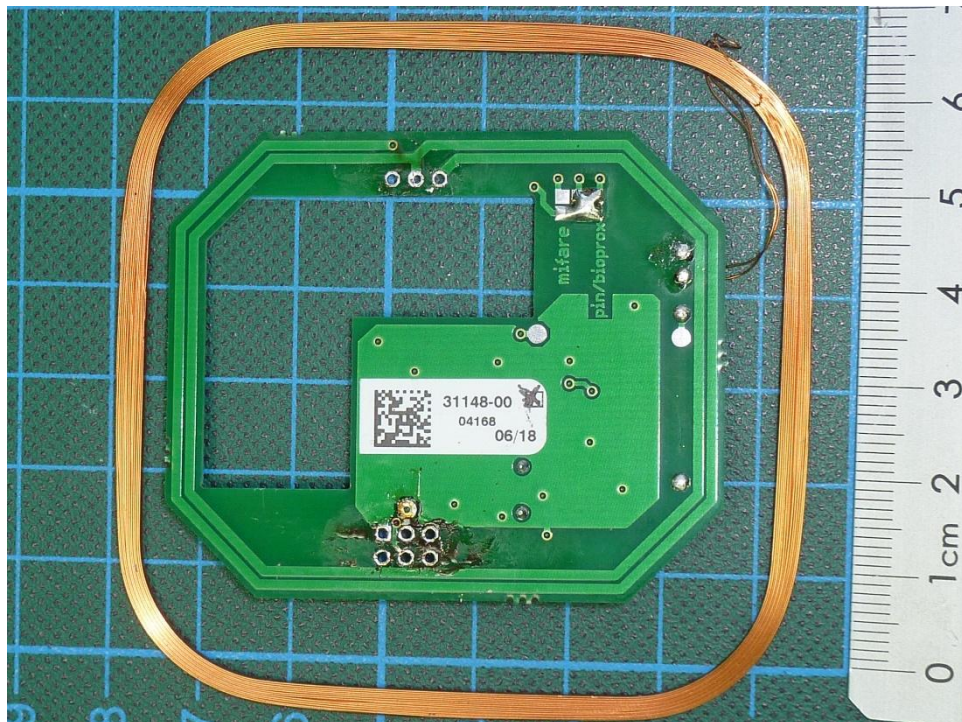
181073eut26: PRD5/2 PCB1 top view
