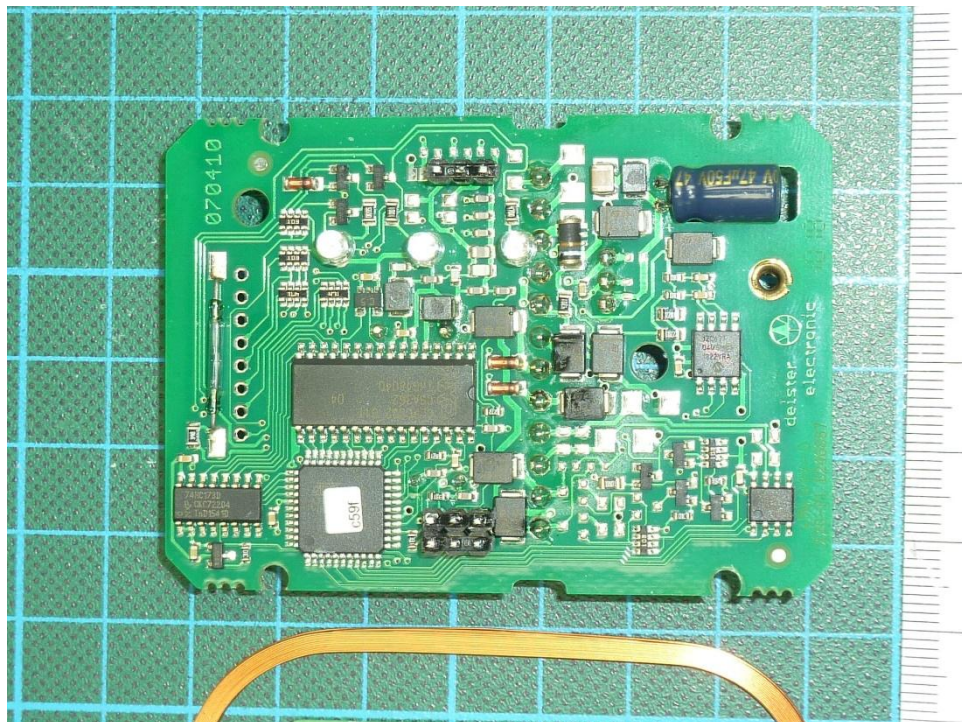
181073eut24: PRD5/2 PCB2 top view
