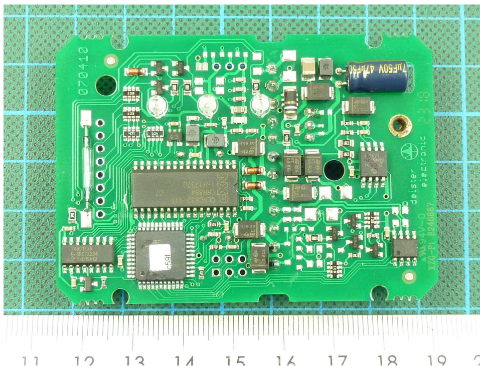
181073eut14.JPG: KPD5/2 PCB 2 top view
