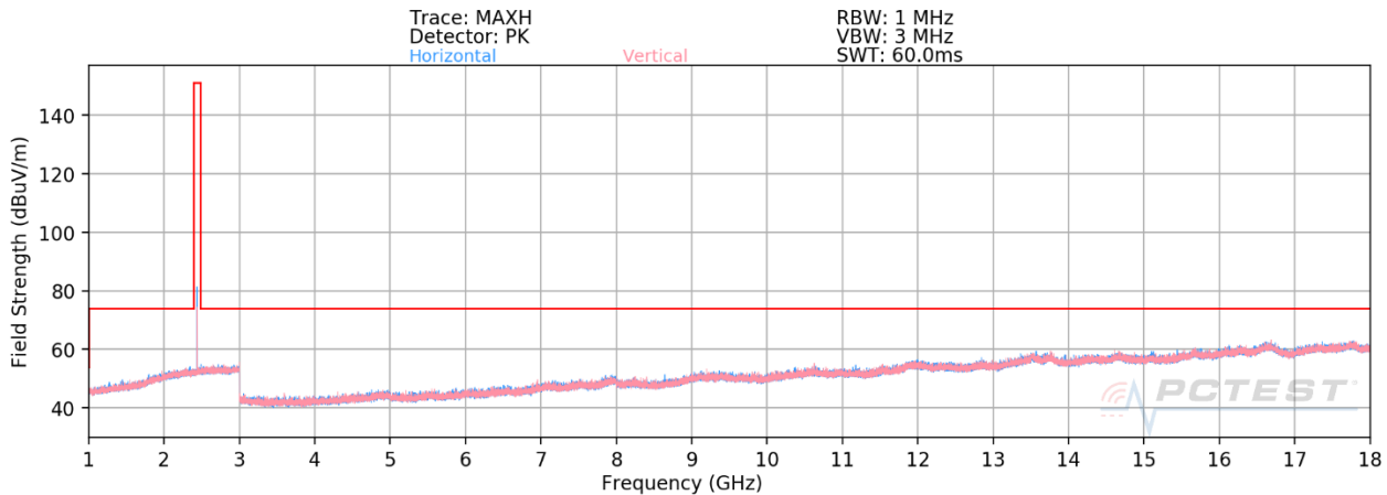
Plot 7-16. Radiated Spurious Emissions Pre-Scan 1-18GHz (1Mbps, Ch. 19)
