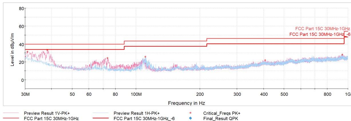
Plot 7-22. Radiated Spurious Emissions Pre-Scan 30MHz-1GHz (1Mbps, Ch.19, with AC/DC Adapter)
