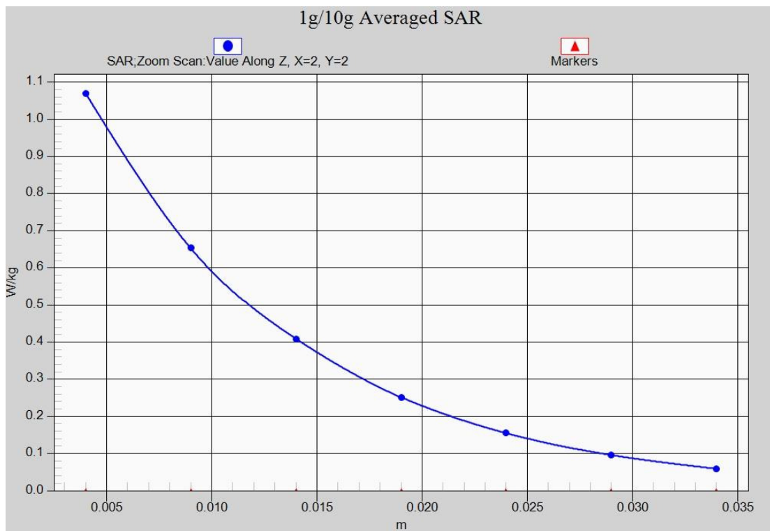
Fig.12-1 Z-Scan at power reference point (Band 2 CH19100)
