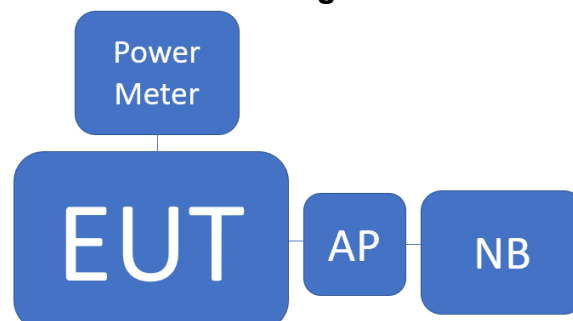
Fig. 2-2 Conducted (Antenna Port) Emission Configuration
