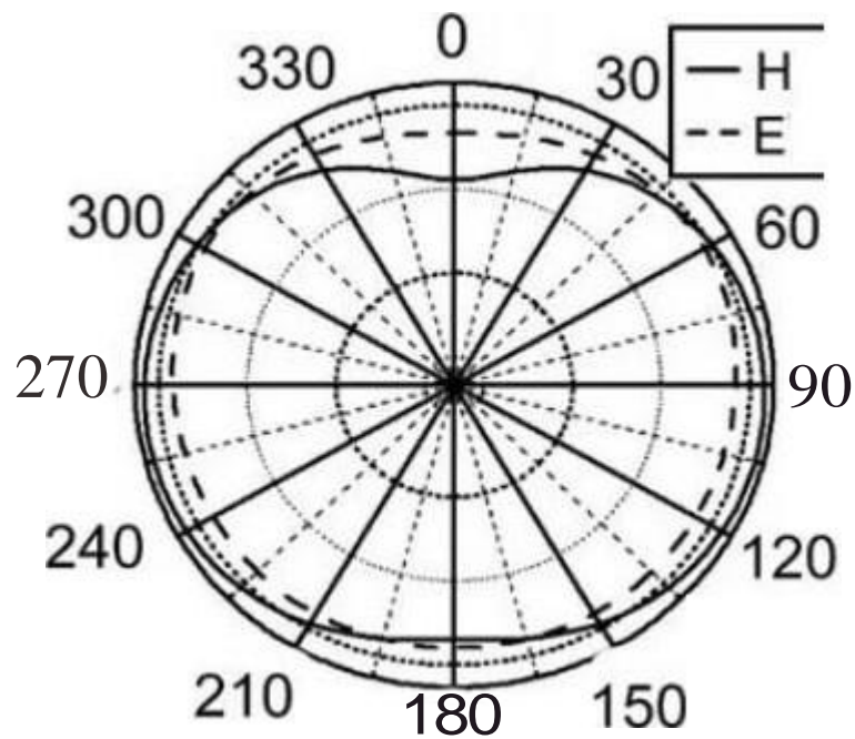
49.860 MHz radiation pattern
