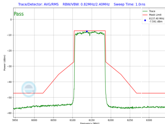
Plot 7-1108. LPI In-Band Emission Plot SDM Diversity Antenna WF7 (80MHz 802.11ax (UNII Band 5) – Ch. 39, MCS2)
