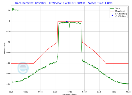
Plot 7-1167. SP In-Band Emission Plot CDD Diversity Antenna WF7 (40MHz 802.11ax (UNII Band 7) – Ch. 155, MCS4)
