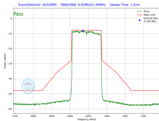
Plot 7-1120. LPI In-Band Emission Plot SDM Diversity Antenna WF7 (80MHz 802.11ax (UNII Band 8) – Ch. 199, MCS2)
