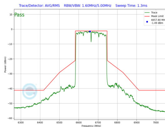
Plot 7-1177. SP In-Band Emission Plot CDD Diversity Antenna WF7 (160MHz 802.11ax (UNII Band 7) – Ch. 143, MCS11)
