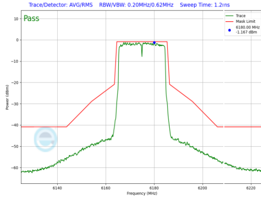
Plot 7-1162. SP In-Band Emission Plot CDD Diversity Antenna WF7 (20MHz 802.11ax (UNII Band 5) – Ch. 45, MCS4)
