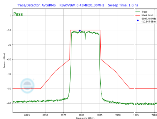
Plot 7-1119. LPI In-Band Emission Plot SDM Diversity Antenna WF7 (40MHz 802.11ax (UNII Band 8) – Ch. 211, MCS2)
