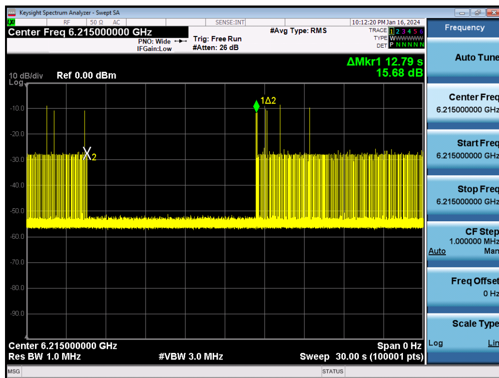
Plot 7-1194. Contention Based Protocol Timing Plot – UNII 5 – 20MHz Channel 53
