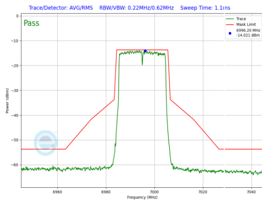
Plot 7-1118. LPI In-Band Emission Plot SDM Diversity Antenna WF7 (20MHz 802.11ax (UNII Band 8) – Ch. 209, MCS2)
