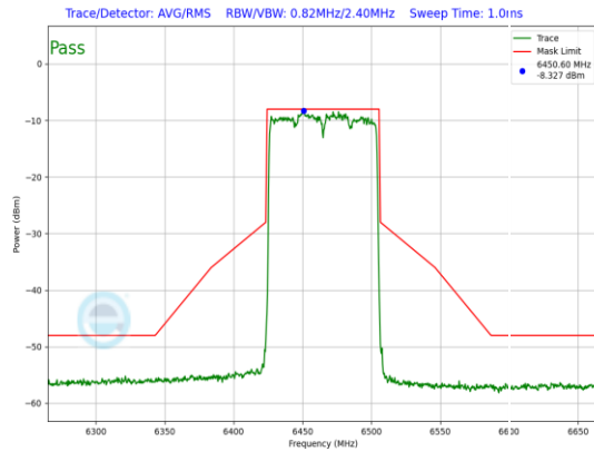
Plot 7-1144. LPI In-Band Emission Plot SDM Diversity Antenna WF7 (80MHz 802.11ax (UNII Band 6) – Ch. 103, MCS11)
