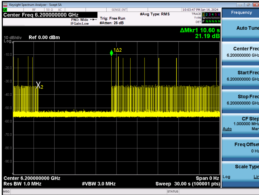
Plot 7-1195. Contention Based Protocol Timing Plot – UNII 5 – 160MHz Channel 47 – Low
