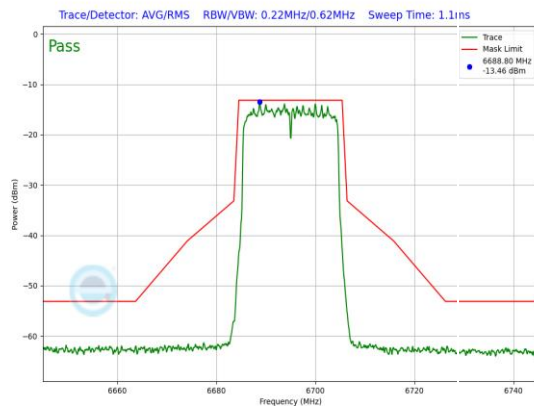
Plot 7-1146. LPI In-Band Emission Plot SDM Diversity Antenna WF7 (20MHz 802.11ax (UNII Band 7) – Ch. 149, MCS11)
