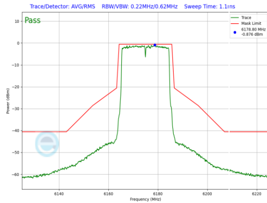
Plot 7-1154. SP In-Band Emission Plot CDD Diversity Antenna WF7 (20MHz 802.11ax (UNII Band 5) – Ch. 45, MCS2)
