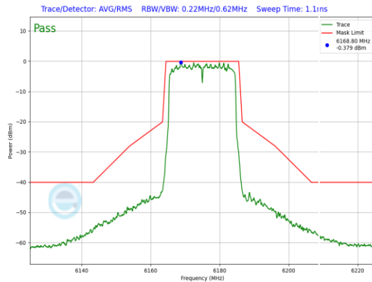
Plot 7-1170. SP In-Band Emission Plot CDD Diversity Antenna WF7 (20MHz 802.11ax (UNII Band 5) – Ch. 45, MCS11)
