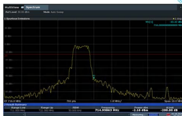
LTE Band85 16QAM 10MHz CH-High, 1 RB
