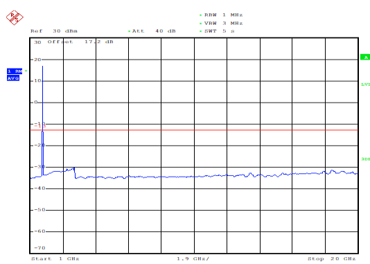
LTE Band 4 1.4MHz CH-Low 1GHz ~20GHz
