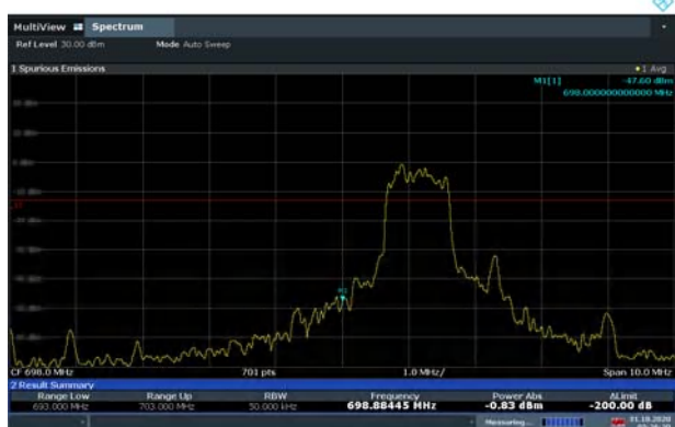
LTE Band 85 16QAM 10MHz CH-Low, 100%RB
