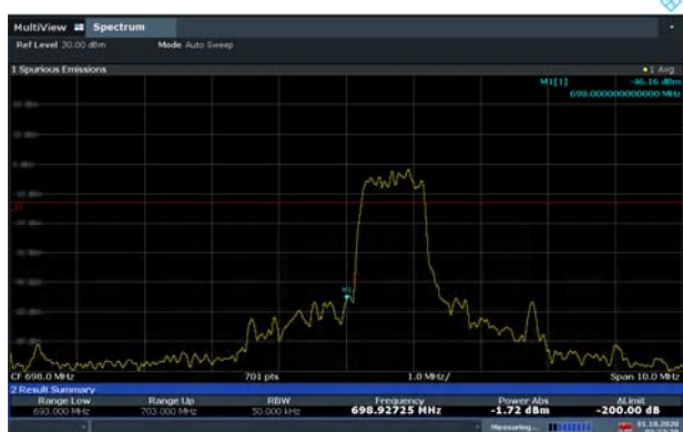
LTE Band 85 16QAM 10MHz CH-Low, 1 RB
