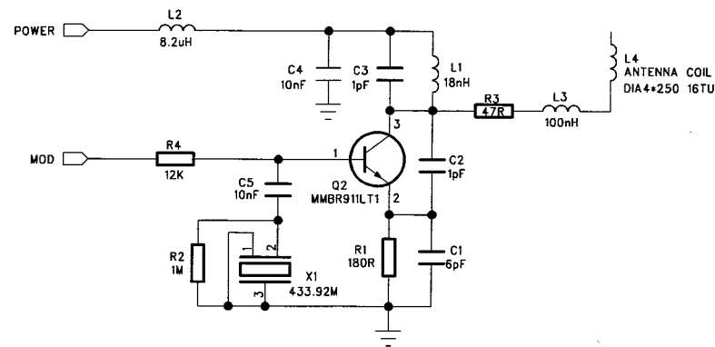
UHF TRANSMITTER
