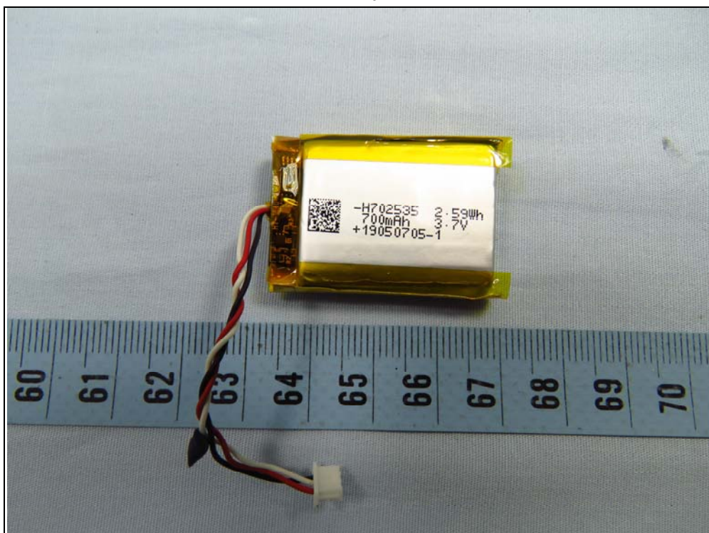
Battery 2
