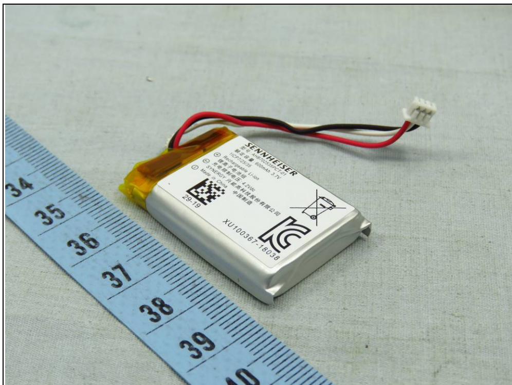
Battery 1
