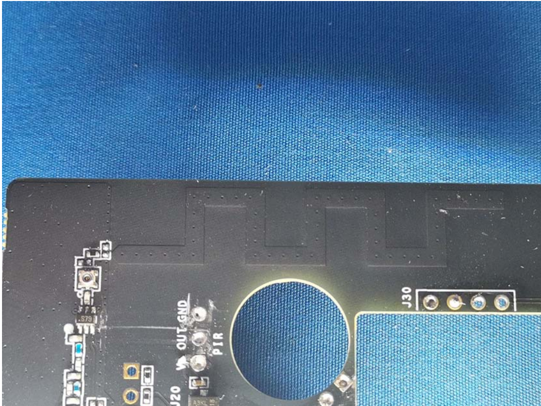
915M Antenna
