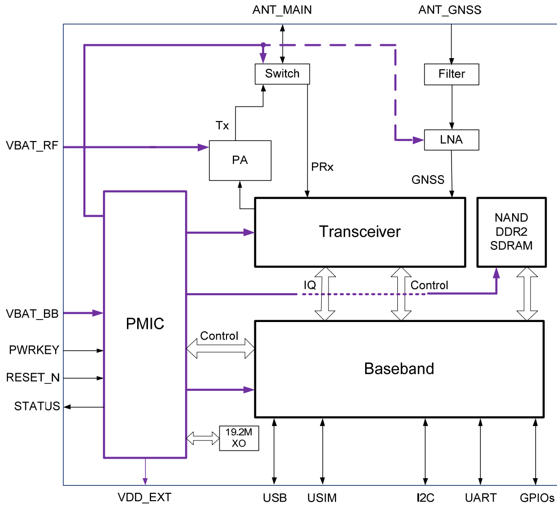
Figure 1: Functional Diagram
