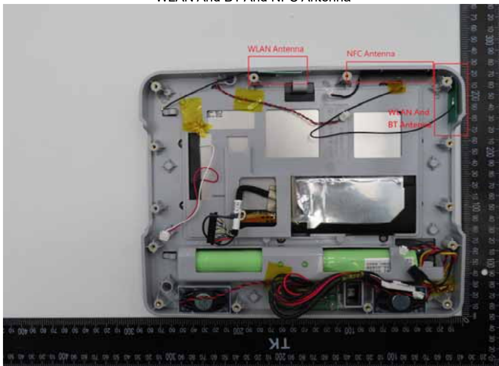
BT+WLAN Antenna
