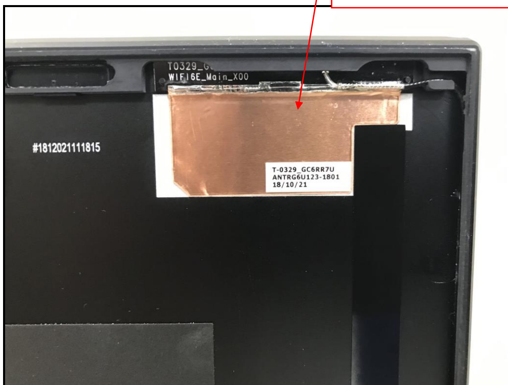
WIFI+BT Antenna (MAIN)
