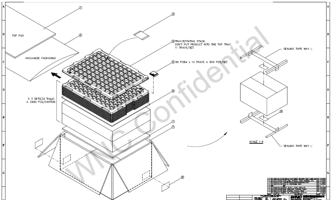
Fig. 10: DN SA-141 Package Drawing
