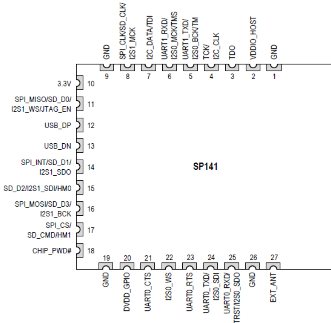
Fig.3: DNSA-141 Pinout (Top side)
