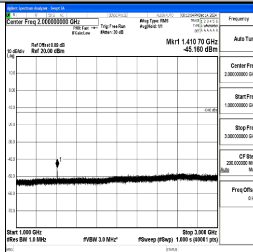
Band12_5MHz_QPSK_23095_1RB#0_1000~3000_1000~3000
