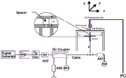
Figure 8-1 System Verification Setup Diagram
