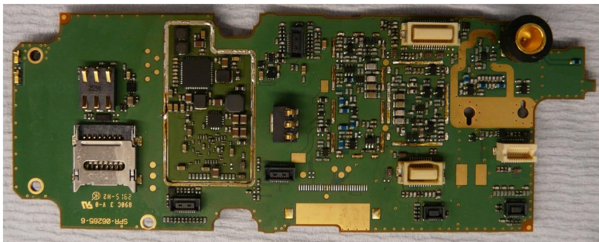
Figure 7. SC2024 Main PCB Top View with Cans Removed
