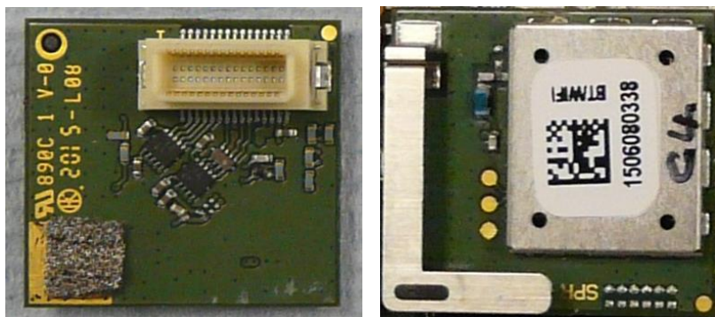
Figure 14. SC2024 Bluetooth/Wi-Fi Module
