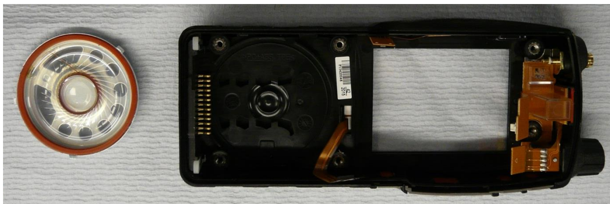
Figure 13. SC2024 Front Cover with Speaker Removed
