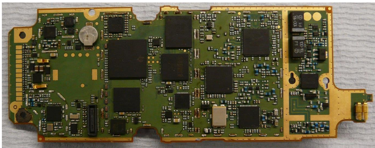
Figure 8. SC2024 Main PCB Bottom View with Cans Removed
