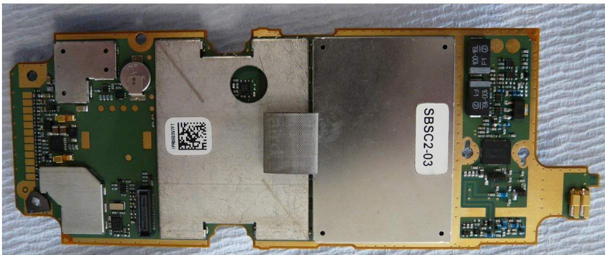
Figure 6. SC2024 Main PCB Bottom View
