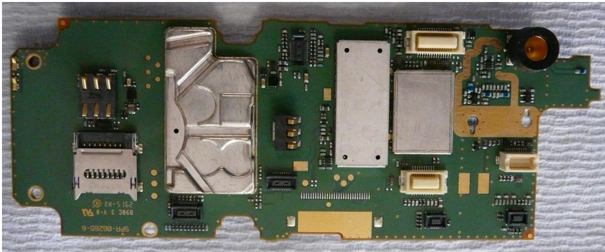
Figure 5. SC2024 Main PCB Top View
