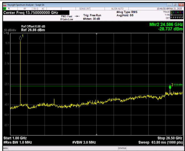
Band7-20MHz-64QAM-21100-1RB#0-Range2:1000~26500MHz
