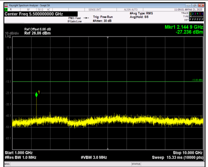
Band12-1.4MHz-16QAM-23017-1RB#0-Range2:1000~10000MHz
