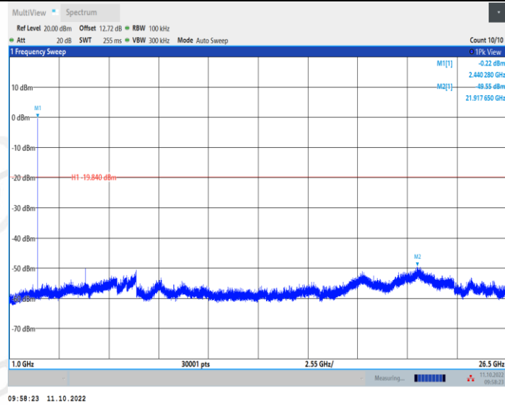
BLE_1M_Ant1_2480_0~Reference
