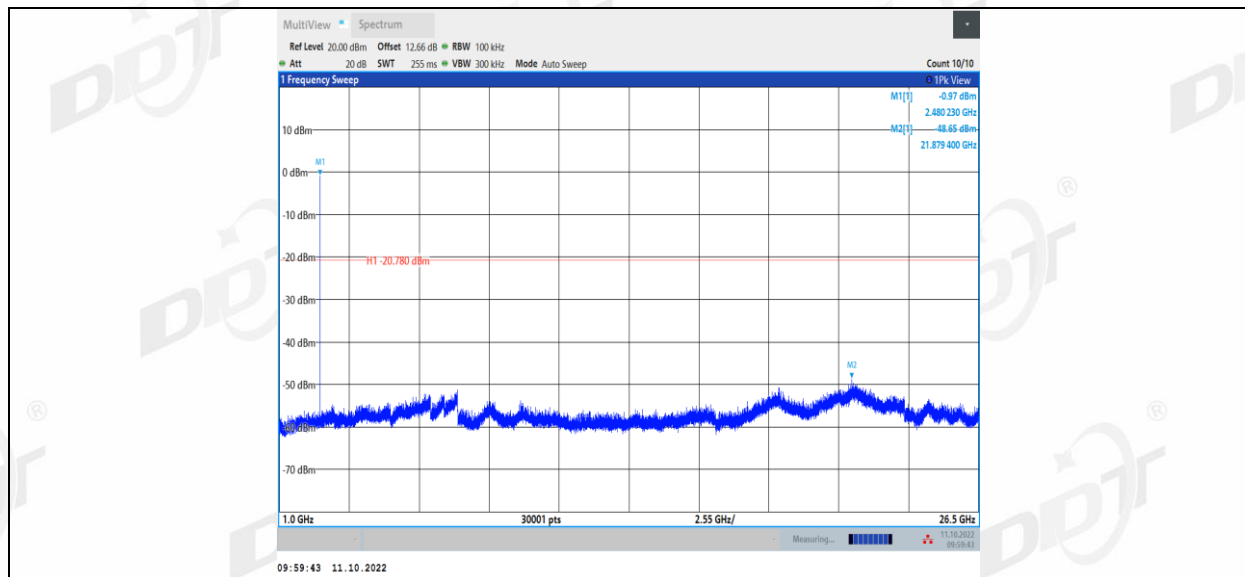
BLE_2M_Ant1_2402_0~Reference
